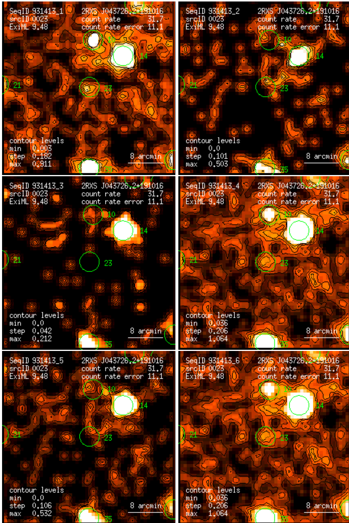
Figure 23: RASS 931413: detection 0023: band rate images, Gaussian filter: (1) PSPC channels 11 – 41, (2) 52 – 90, (3) 91 – 201, (4) 11 – 235, (5) 52 – 201, (6) 11 – 201. Broad band rates in counts/ks. Band rate contour levels in counts/ks/arcmin 2 .
