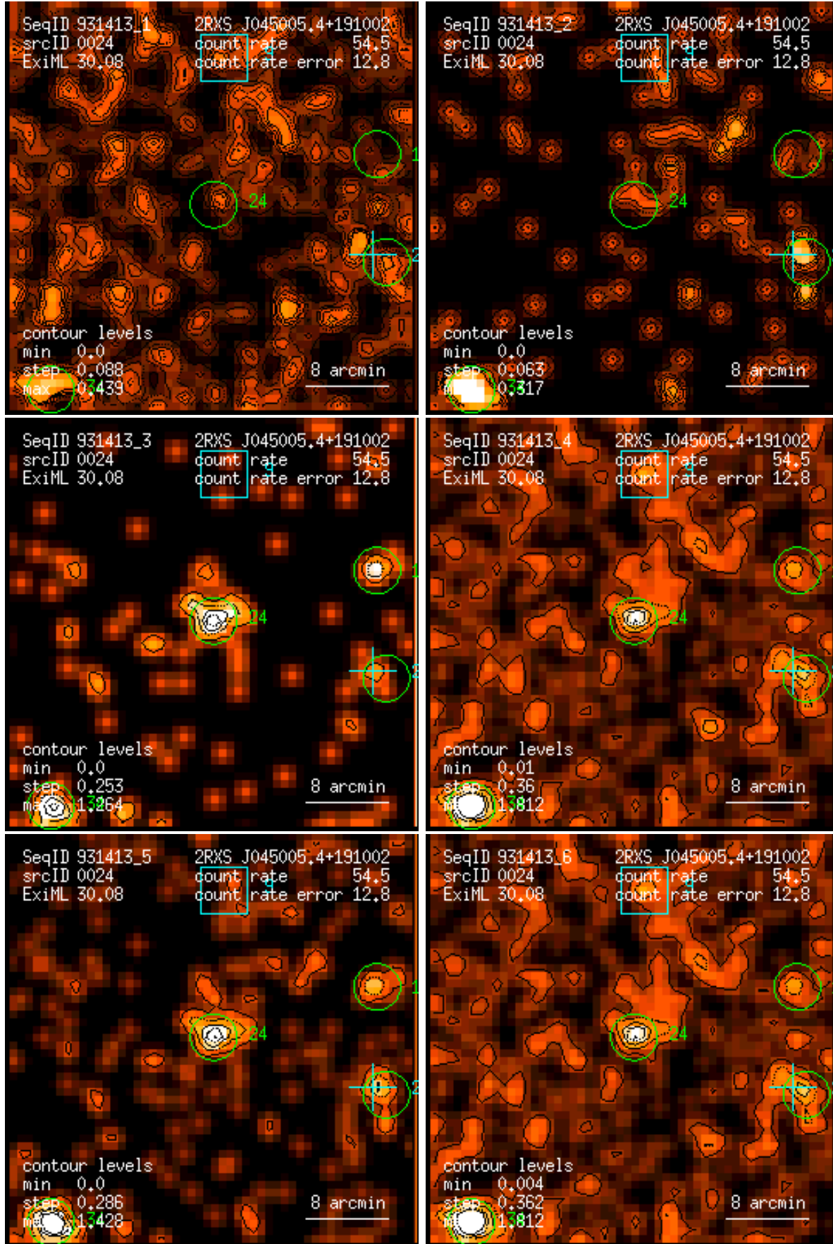
Figure 24: RASS 931413: detection 0024: band rate images, Gaussian filter: (1) PSPC channels 11 – 41, (2) 52 – 90, (3) 91 – 201, (4) 11 – 235, (5) 52 – 201, (6) 11 – 201. Broad band rates in counts/ks. Band rate contour levels in counts/ks/arcmin 2 .
