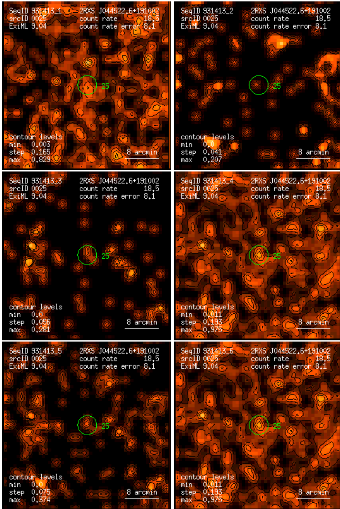
Figure 25: RASS 931413: detection 0025: band rate images, Gaussian filter: (1) PSPC channels 11 – 41, (2) 52 – 90, (3) 91 – 201, (4) 11 – 235, (5) 52 – 201, (6) 11 – 201. Broad band rates in counts/ks. Band rate contour levels in counts/ks/arcmin 2 .
