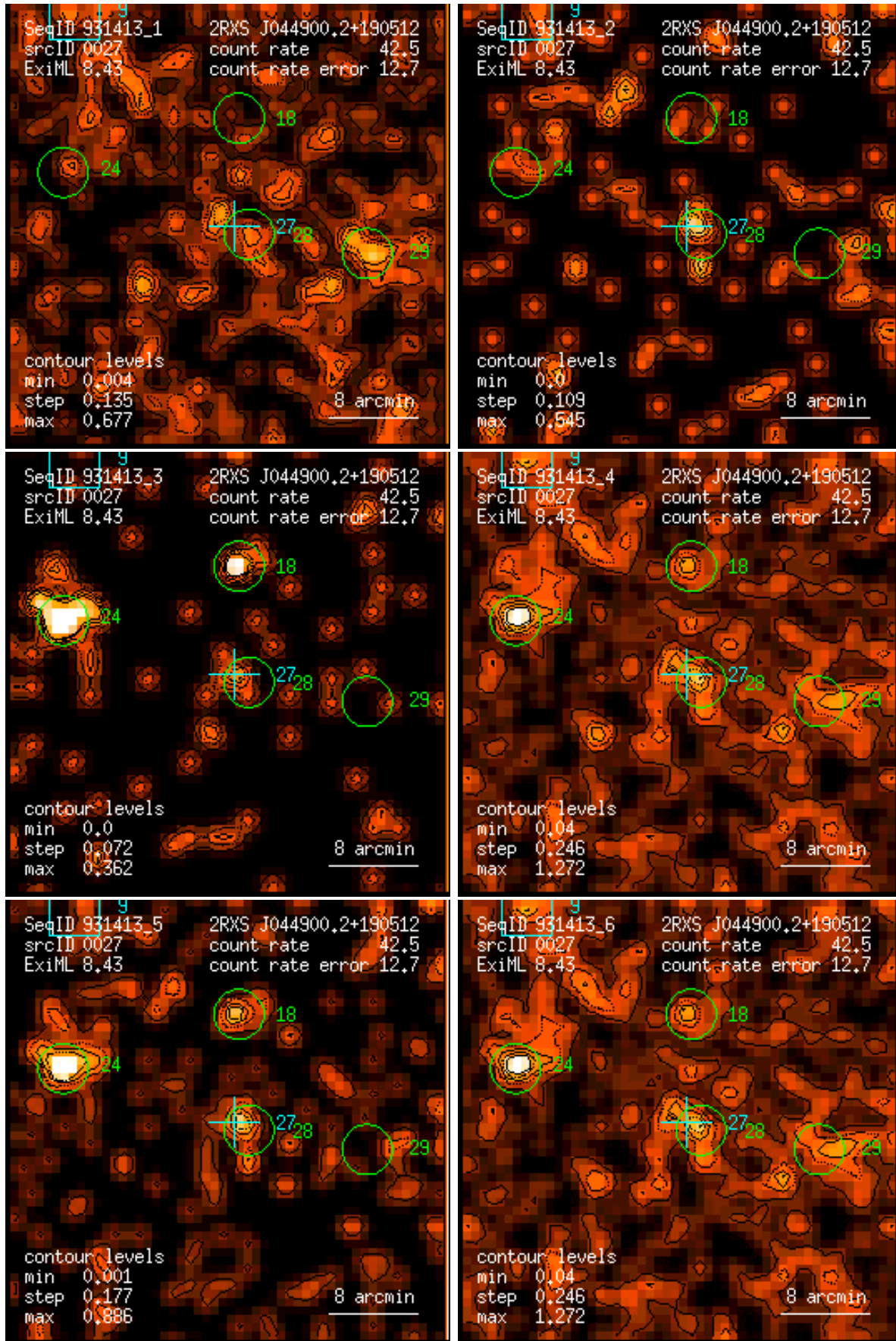
Figure 27: RASS 931413: detection 0027: band rate images, Gaussian filter: (1) PSPC channels 11 – 41, (2) 52 – 90, (3) 91 – 201, (4) 11 – 235, (5) 52 – 201, (6) 11 – 201. Broad band rates in counts/ks. Band rate contour levels in counts/ks/arcmin 2 .
