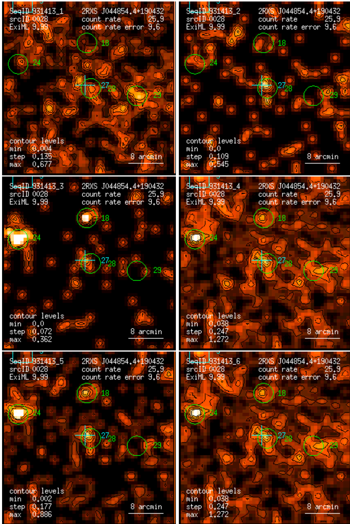
Figure 28: RASS 931413: detection 0028: band rate images, Gaussian filter: (1) PSPC channels 11 – 41, (2) 52 – 90, (3) 91 – 201, (4) 11 – 235, (5) 52 – 201, (6) 11 – 201. Broad band rates in counts/ks. Band rate contour levels in counts/ks/arcmin 2 .
