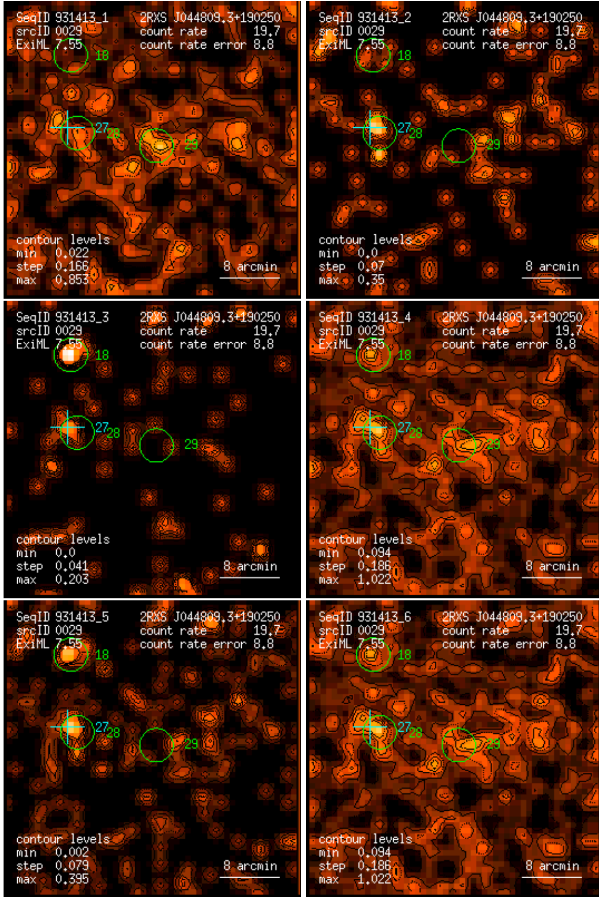
Figure 29: RASS 931413: detection 0029: band rate images, Gaussian filter: (1) PSPC channels 11 – 41, (2) 52 – 90, (3) 91 – 201, (4) 11 – 235, (5) 52 – 201, (6) 11 – 201. Broad band rates in counts/ks. Band rate contour levels in counts/ks/arcmin 2 .
