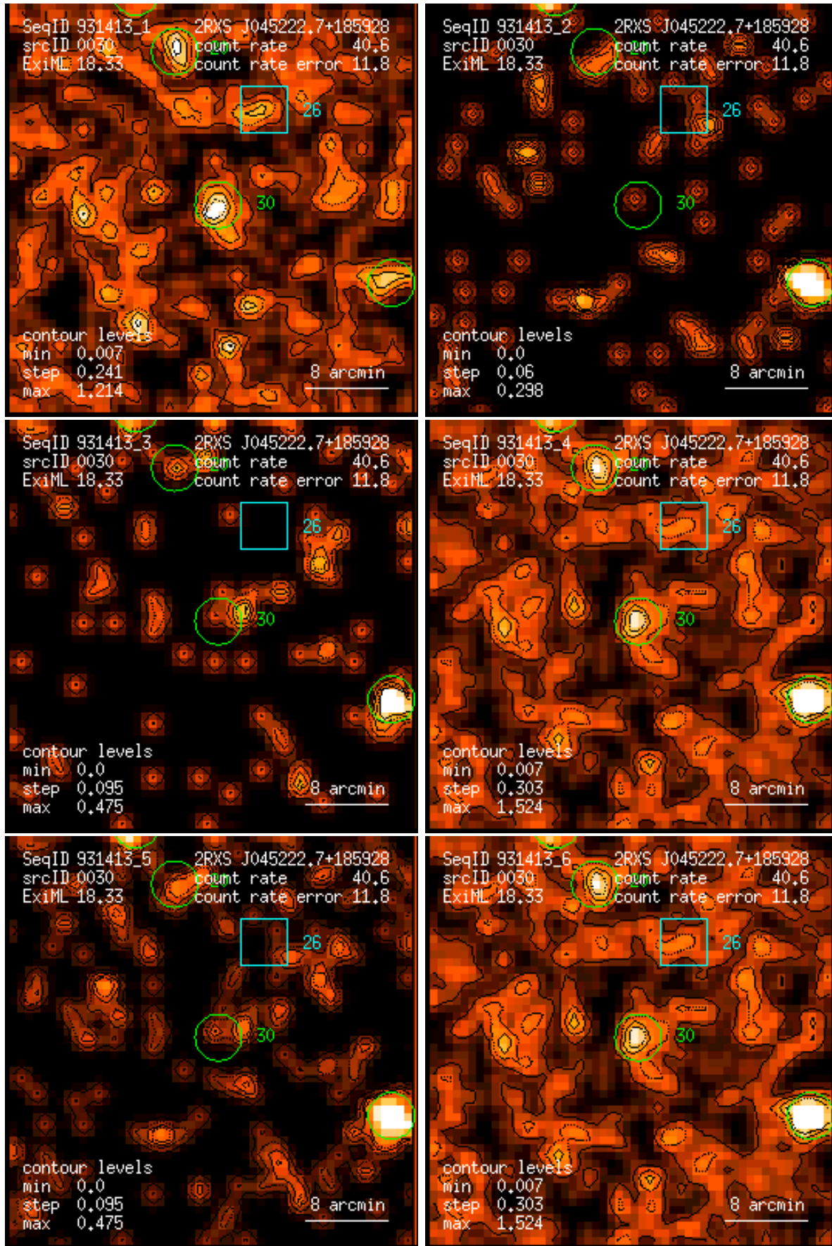
Figure 30: RASS 931413: detection 0030: band rate images, Gaussian filter: (1) PSPC channels 11 – 41, (2) 52 – 90, (3) 91 – 201, (4) 11 – 235, (5) 52 – 201, (6) 11 – 201. Broad band rates in counts/ks. Band rate contour levels in counts/ks/arcmin 2 .
