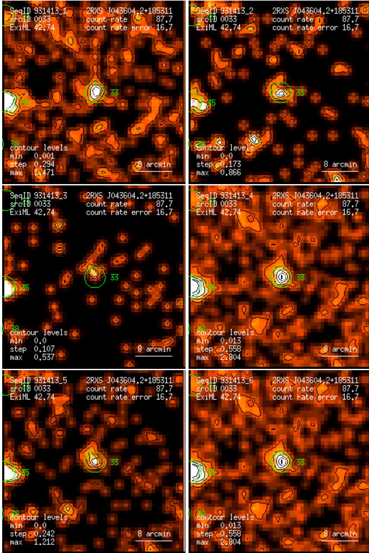
Figure 33: RASS 931413: detection 0033: band rate images, Gaussian filter: (1) PSPC channels 11 – 41, (2) 52 – 90, (3) 91 – 201, (4) 11 – 235, (5) 52 – 201, (6) 11 – 201. Broad band rates in counts/ks. Band rate contour levels in counts/ks/arcmin 2 .
