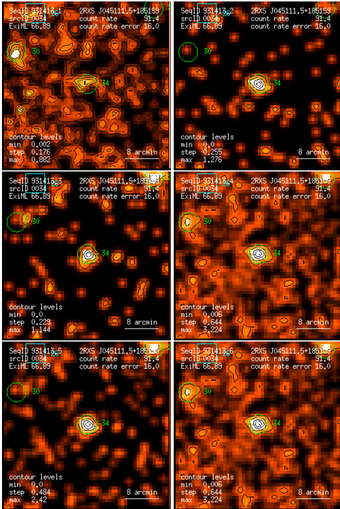
Figure 34: RASS 931413: detection 0034: band rate images, Gaussian filter: (1) PSPC channels 11 – 41, (2) 52 – 90, (3) 91 – 201, (4) 11 – 235, (5) 52 – 201, (6) 11 – 201. Broad band rates in counts/ks. Band rate contour levels in counts/ks/arcmin 2 .
