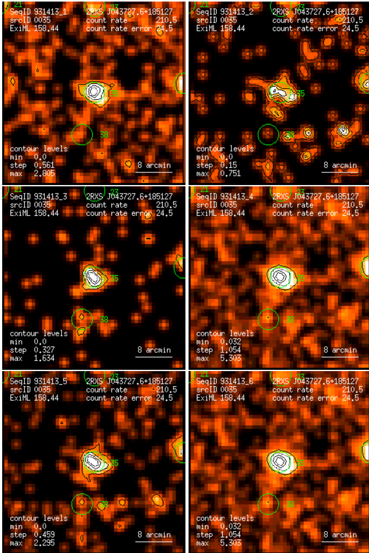
Figure 35: RASS 931413: detection 0035: band rate images, Gaussian filter: (1) PSPC channels 11 – 41, (2) 52 – 90, (3) 91 – 201, (4) 11 – 235, (5) 52 – 201, (6) 11 – 201. Broad band rates in counts/ks. Band rate contour levels in counts/ks/arcmin 2 .
