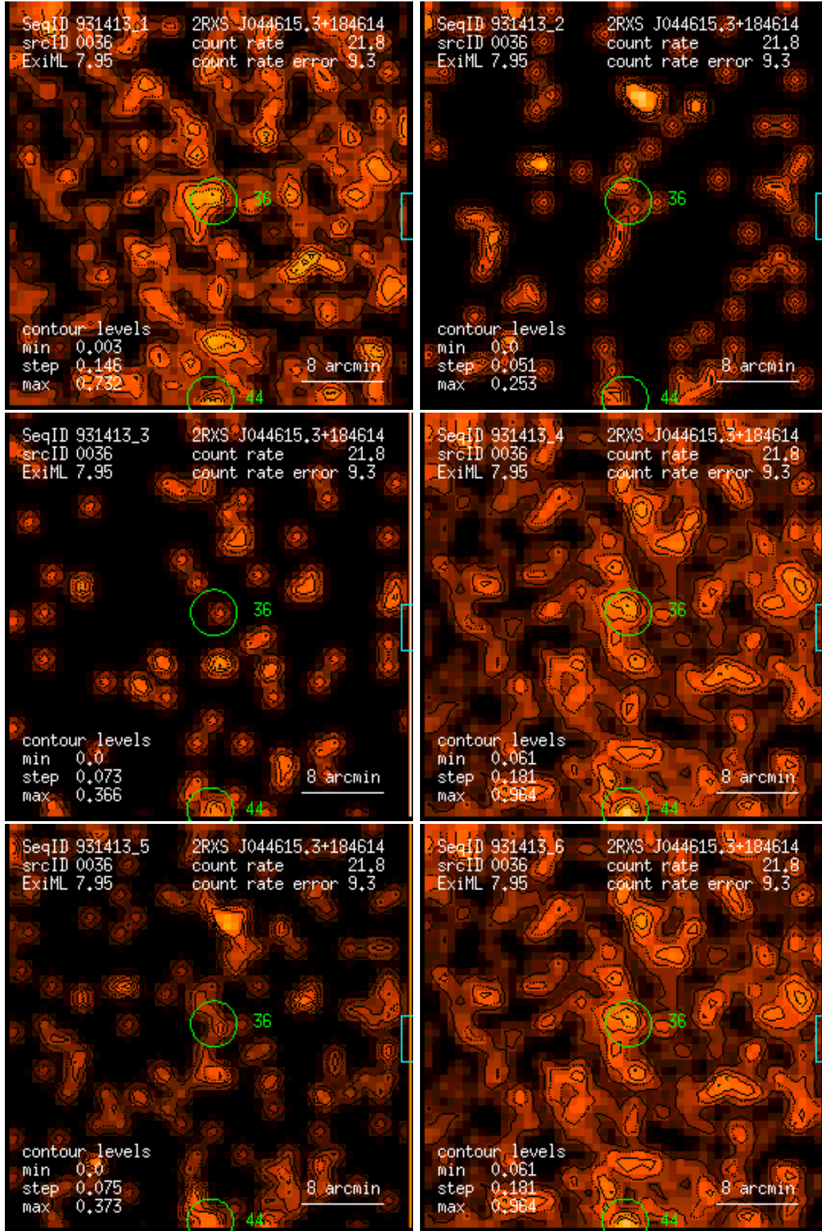
Figure 36: RASS 931413: detection 0036: band rate images, Gaussian filter: (1) PSPC channels 11 – 41, (2) 52 – 90, (3) 91 – 201, (4) 11 – 235, (5) 52 – 201, (6) 11 – 201. Broad band rates in counts/ks. Band rate contour levels in counts/ks/arcmin 2 .
