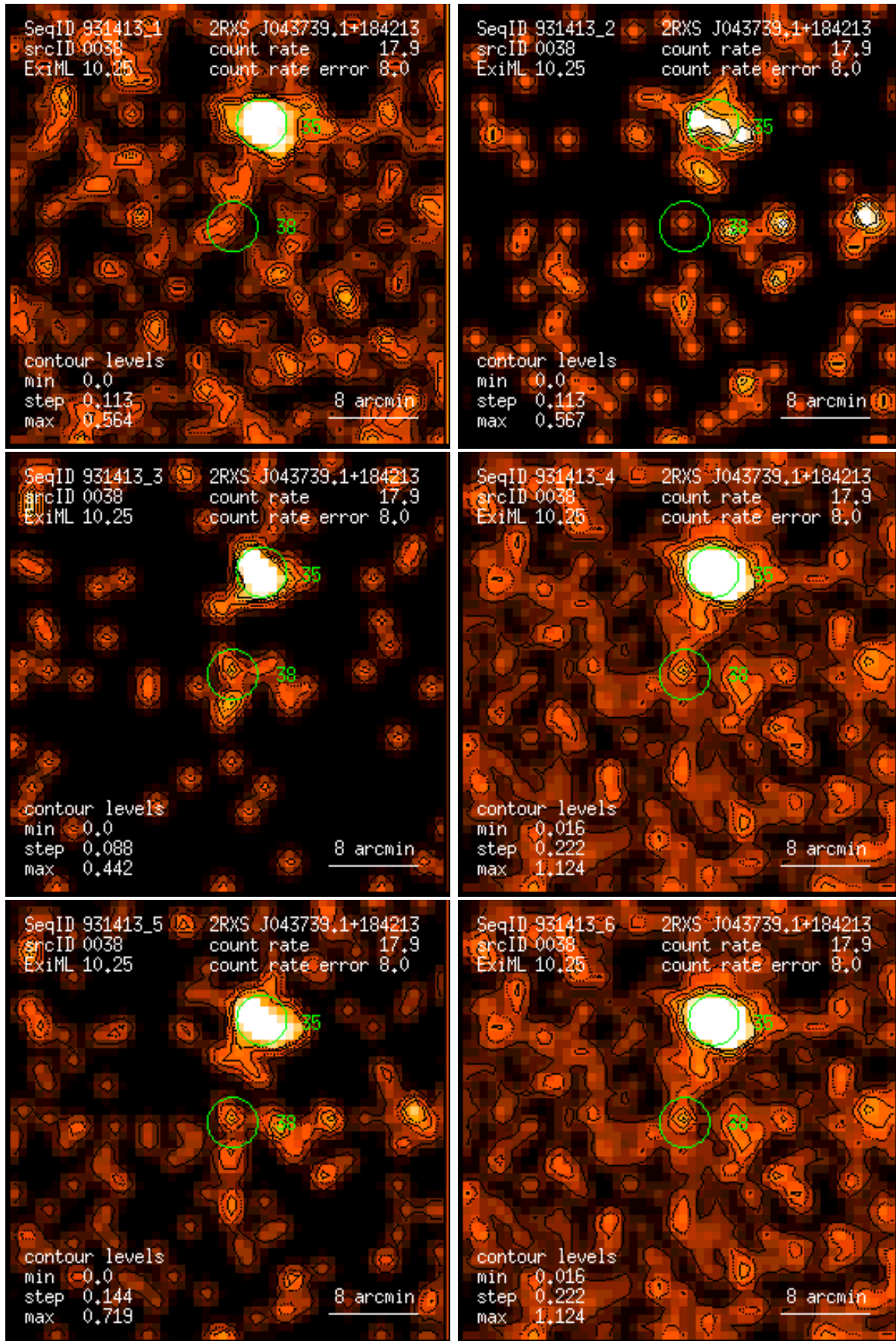
Figure 38: RASS 931413: detection 0038: band rate images, Gaussian filter: (1) PSPC channels 11 – 41, (2) 52 – 90, (3) 91 – 201, (4) 11 – 235, (5) 52 – 201, (6) 11 – 201. Broad band rates in counts/ks. Band rate contour levels in counts/ks/arcmin 2 .
