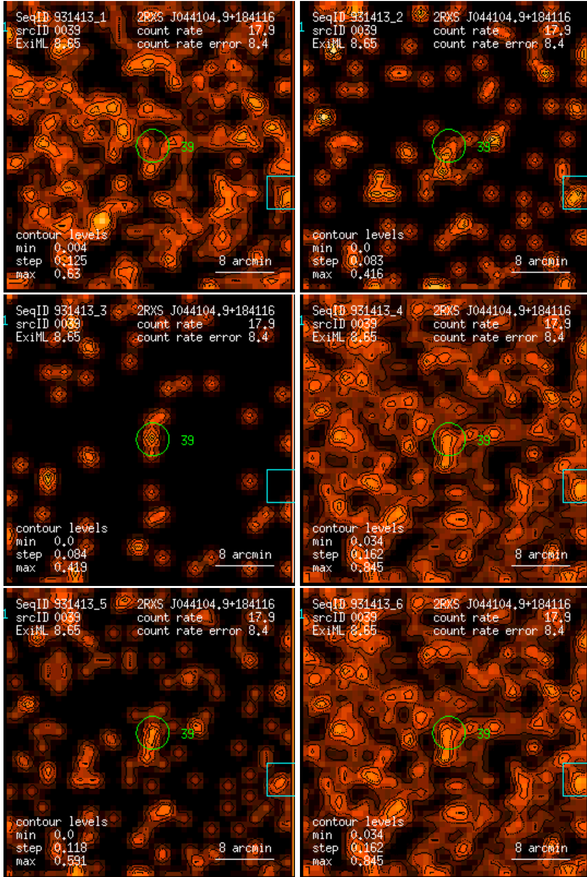
Figure 39: RASS 931413: detection 0039: band rate images, Gaussian filter: (1) PSPC channels 11 – 41, (2) 52 – 90, (3) 91 – 201, (4) 11 – 235, (5) 52 – 201, (6) 11 – 201. Broad band rates in counts/ks. Band rate contour levels in counts/ks/arcmin 2 .
