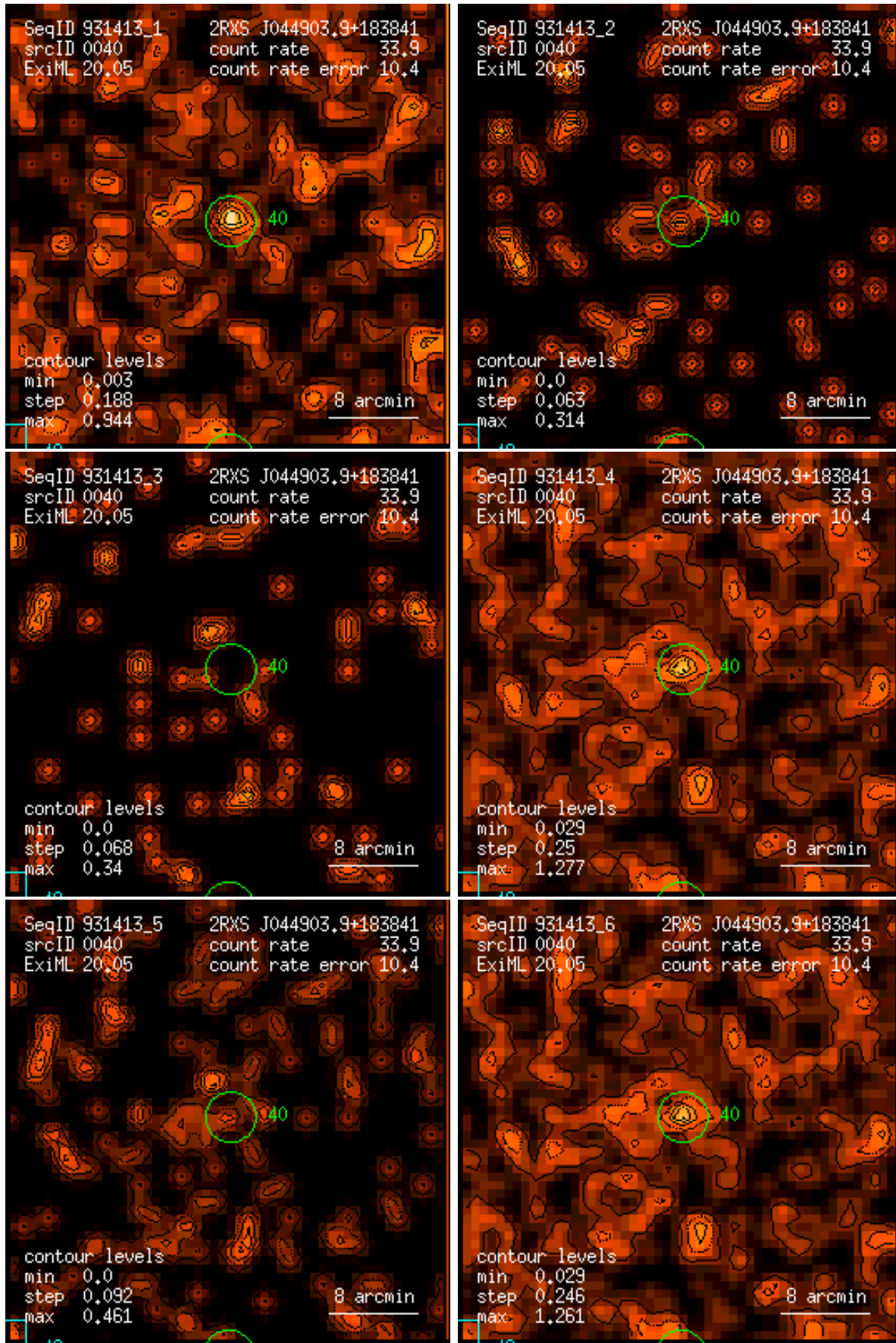
Figure 40: RASS 931413: detection 0040: band rate images, Gaussian filter: (1) PSPC channels 11 – 41, (2) 52 – 90, (3) 91 – 201, (4) 11 – 235, (5) 52 – 201, (6) 11 – 201. Broad band rates in counts/ks. Band rate contour levels in counts/ks/arcmin 2 .
