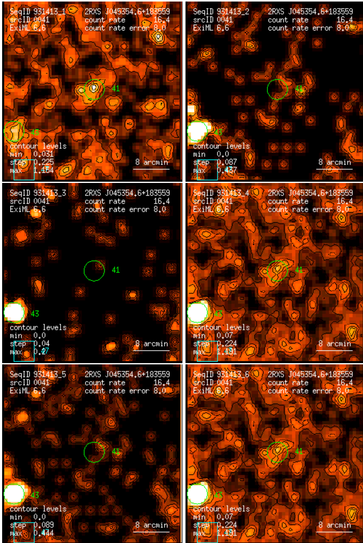
Figure 41: RASS 931413: detection 0041: band rate images, Gaussian filter: (1) PSPC channels 11 – 41, (2) 52 – 90, (3) 91 – 201, (4) 11 – 235, (5) 52 – 201, (6) 11 – 201. Broad band rates in counts/ks. Band rate contour levels in counts/ks/arcmin 2 .
