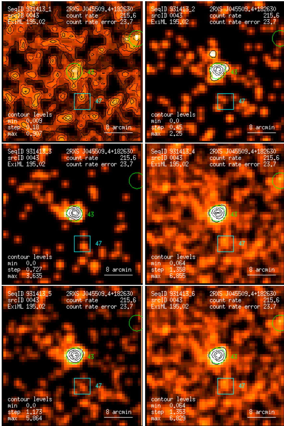
Figure 43: RASS 931413: detection 0043: band rate images, Gaussian filter: (1) PSPC channels 11 – 41, (2) 52 – 90, (3) 91 – 201, (4) 11 – 235, (5) 52 – 201, (6) 11 – 201. Broad band rates in counts/ks. Band rate contour levels in counts/ks/arcmin 2 .
