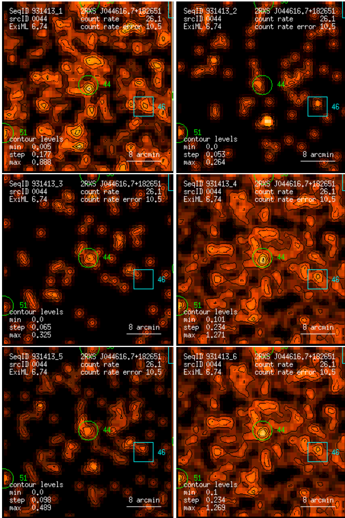
Figure 44: RASS 931413: detection 0044: band rate images, Gaussian filter: (1) PSPC channels 11 – 41, (2) 52 – 90, (3) 91 – 201, (4) 11 – 235, (5) 52 – 201, (6) 11 – 201. Broad band rates in counts/ks. Band rate contour levels in counts/ks/arcmin 2 .
