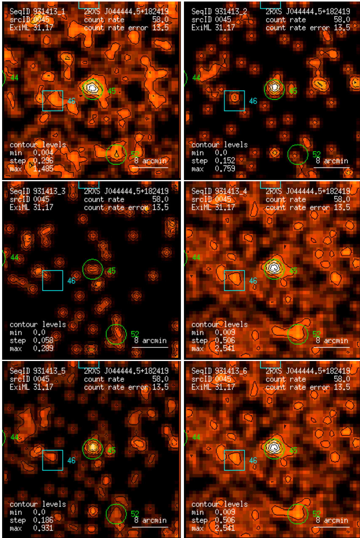
Figure 45: RASS 931413: detection 0045: band rate images, Gaussian filter: (1) PSPC channels 11 – 41, (2) 52 – 90, (3) 91 – 201, (4) 11 – 235, (5) 52 – 201, (6) 11 – 201. Broad band rates in counts/ks. Band rate contour levels in counts/ks/arcmin 2 .
