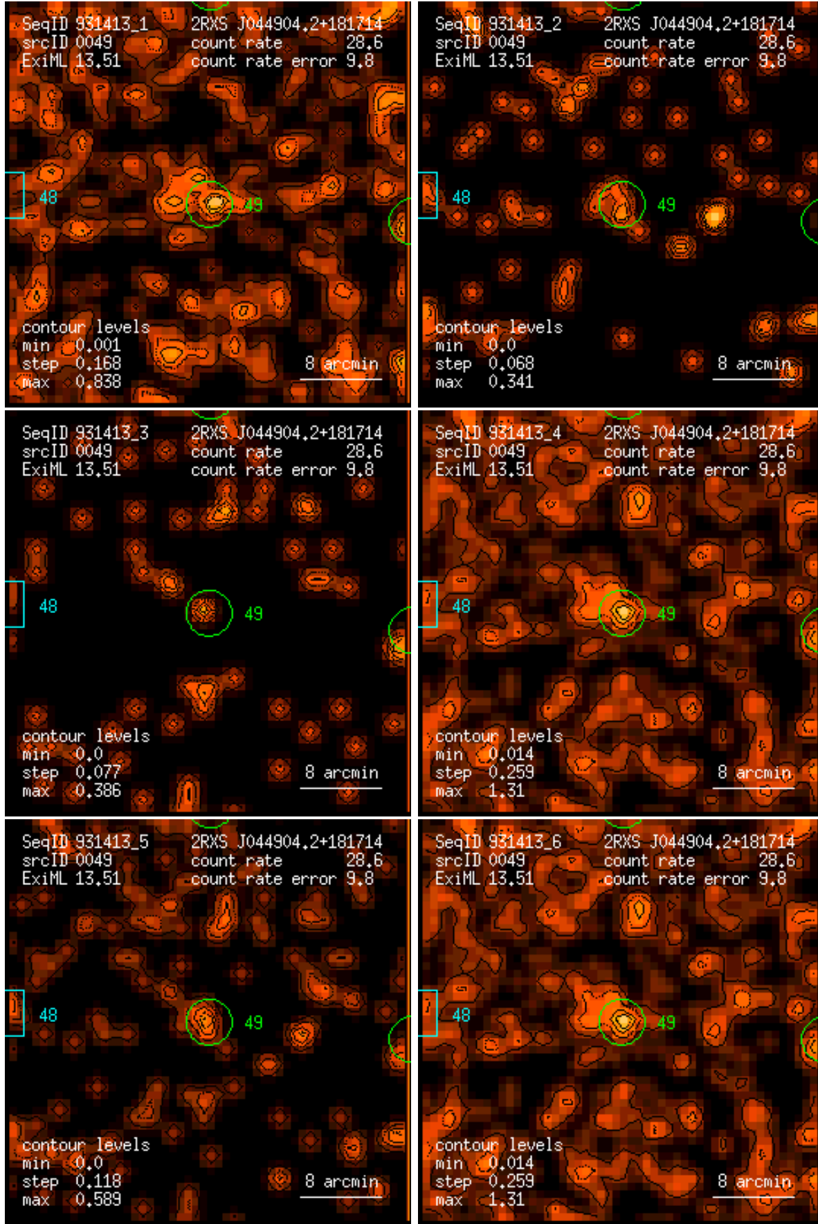
Figure 49: RASS 931413: detection 0049: band rate images, Gaussian filter: (1) PSPC channels 11 – 41, (2) 52 – 90, (3) 91 – 201, (4) 11 – 235, (5) 52 – 201, (6) 11 – 201. Broad band rates in counts/ks. Band rate contour levels in counts/ks/arcmin 2 .
