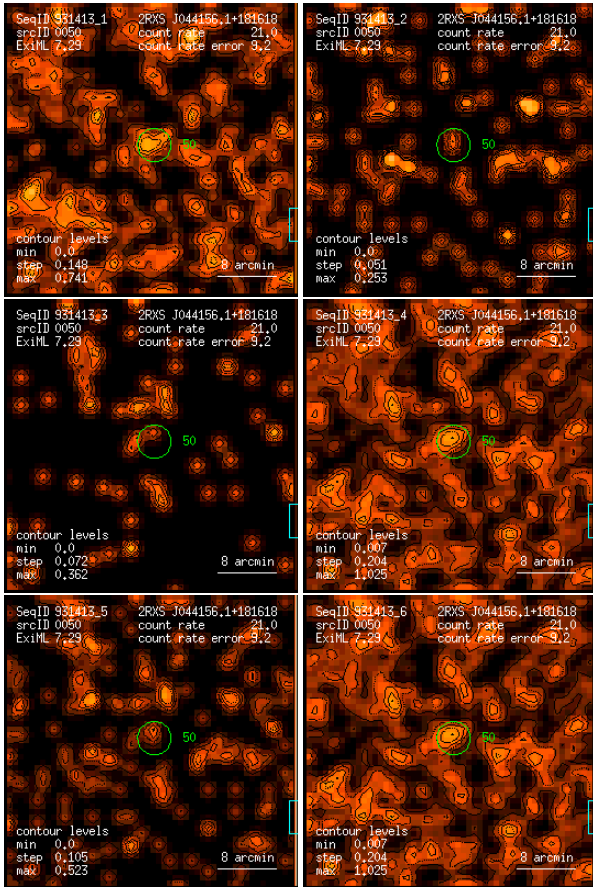
Figure 50: RASS 931413: detection 0050: band rate images, Gaussian filter: (1) PSPC channels 11 – 41, (2) 52 – 90, (3) 91 – 201, (4) 11 – 235, (5) 52 – 201, (6) 11 – 201. Broad band rates in counts/ks. Band rate contour levels in counts/ks/arcmin 2 .
