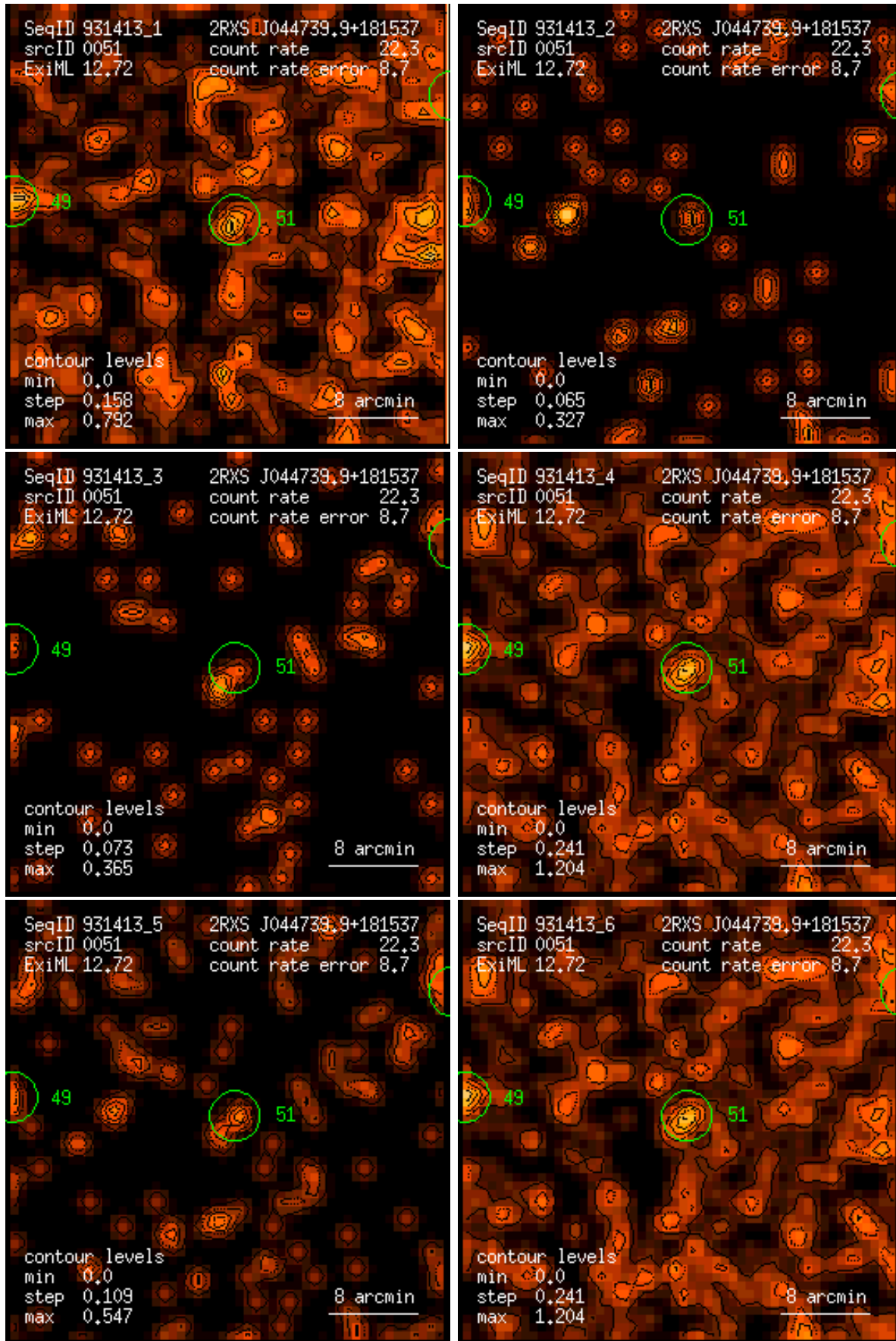
Figure 51: RASS 931413: detection 0051: band rate images, Gaussian filter: (1) PSPC channels 11 – 41, (2) 52 – 90, (3) 91 – 201, (4) 11 – 235, (5) 52 – 201, (6) 11 – 201. Broad band rates in counts/ks. Band rate contour levels in counts/ks/arcmin 2 .
