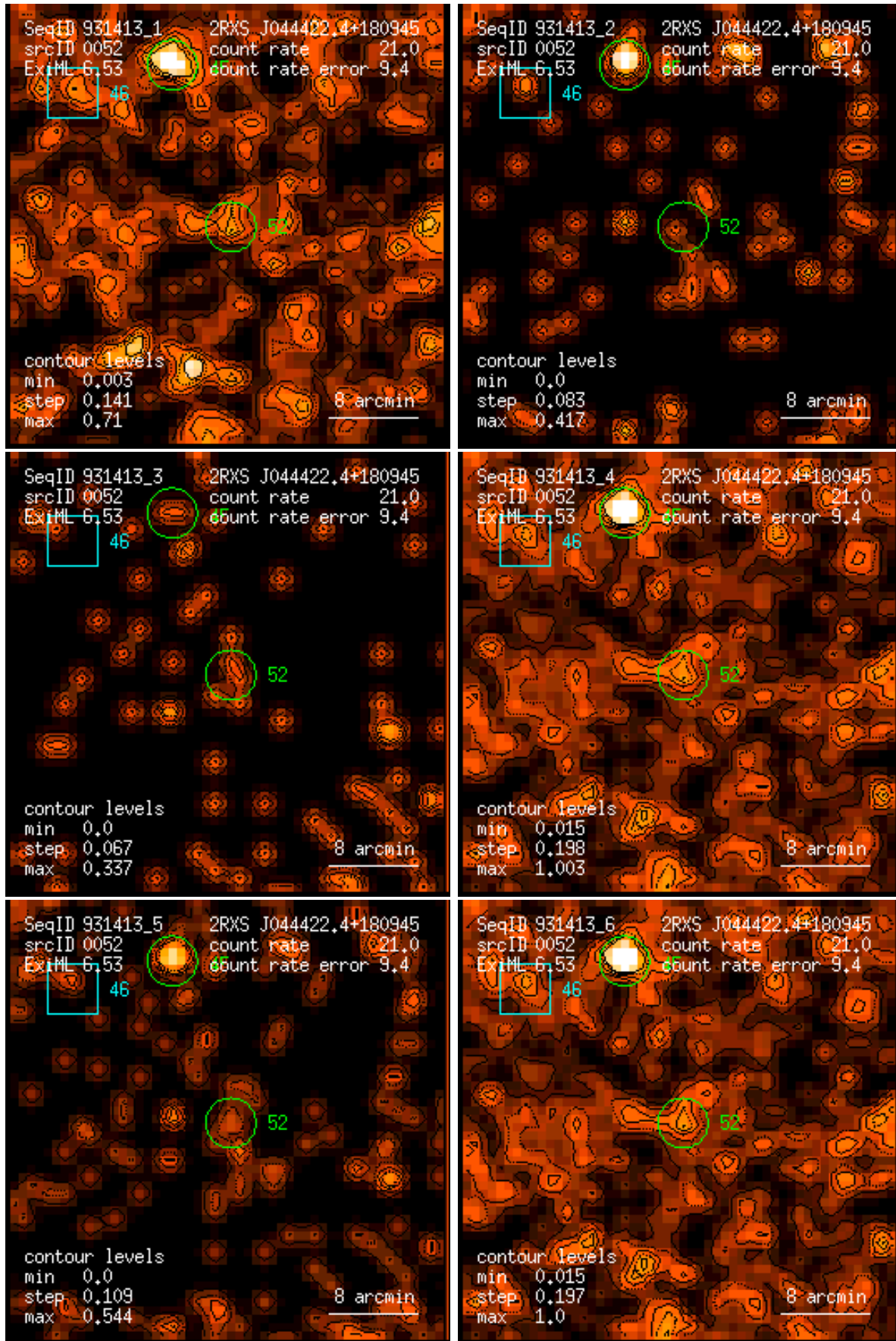
Figure 52: RASS 931413: detection 0052: band rate images, Gaussian filter: (1) PSPC channels 11 – 41, (2) 52 – 90, (3) 91 – 201, (4) 11 – 235, (5) 52 – 201, (6) 11 – 201. Broad band rates in counts/ks. Band rate contour levels in counts/ks/arcmin 2 .
