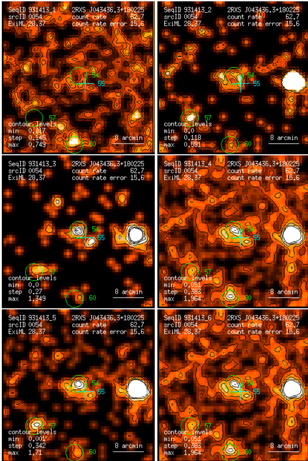
Figure 54: RASS 931413: detection 0054: band rate images, Gaussian filter: (1) PSPC channels 11 – 41, (2) 52 – 90, (3) 91 – 201, (4) 11 – 235, (5) 52 – 201, (6) 11 – 201. Broad band rates in counts/ks. Band rate contour levels in counts/ks/arcmin 2 .
