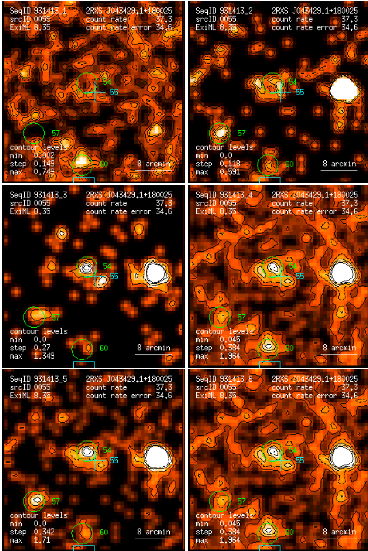
Figure 55: RASS 931413: detection 0055: band rate images, Gaussian filter: (1) PSPC channels 11 – 41, (2) 52 – 90, (3) 91 – 201, (4) 11 – 235, (5) 52 – 201, (6) 11 – 201. Broad band rates in counts/ks. Band rate contour levels in counts/ks/arcmin 2 .
