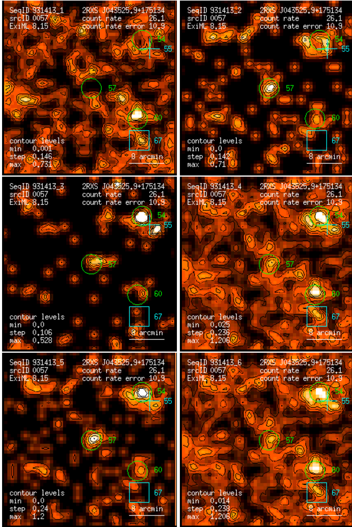
Figure 57: RASS 931413: detection 0057: band rate images, Gaussian filter: (1) PSPC channels 11 – 41, (2) 52 – 90, (3) 91 – 201, (4) 11 – 235, (5) 52 – 201, (6) 11 – 201. Broad band rates in counts/ks. Band rate contour levels in counts/ks/arcmin 2 .
