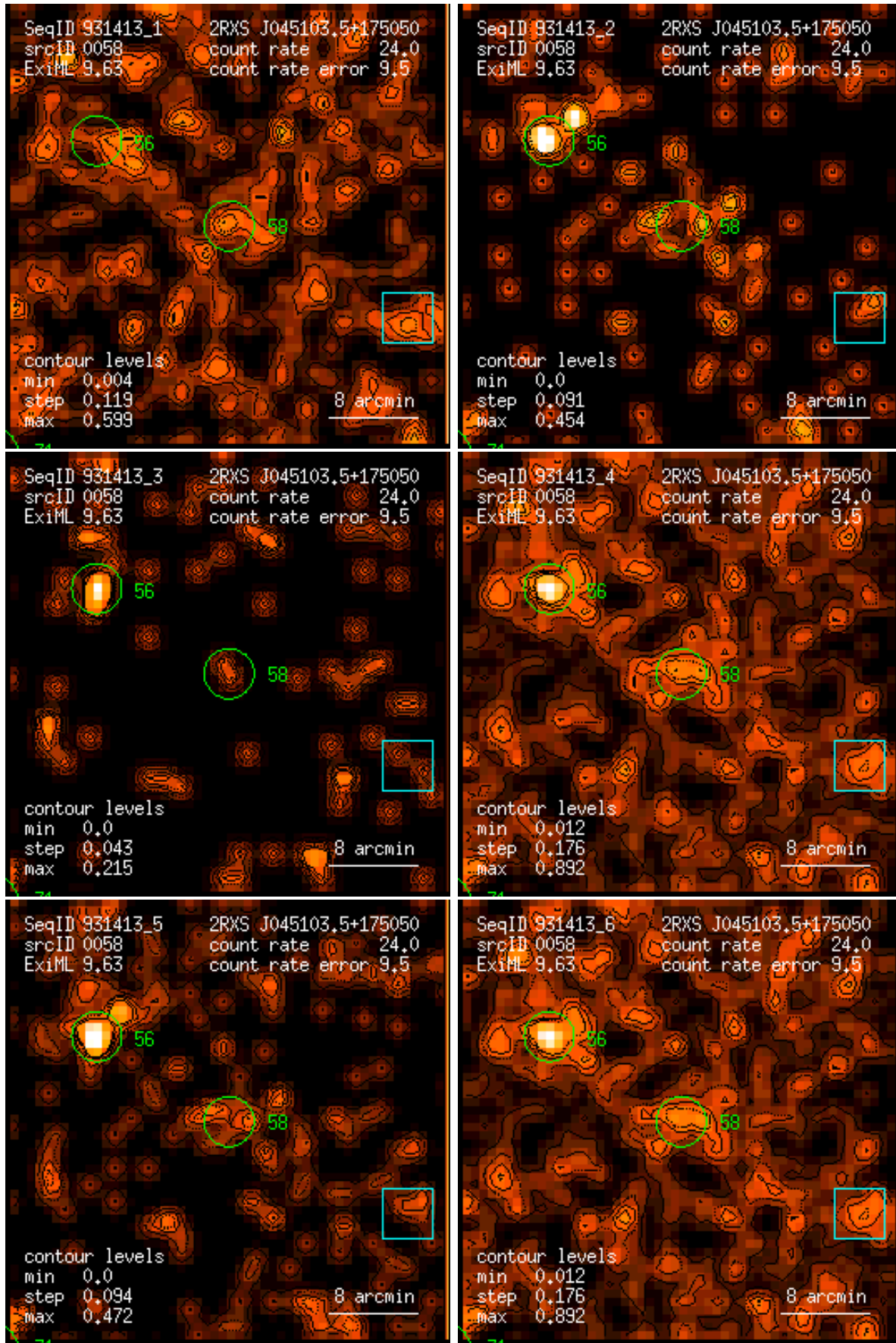
Figure 58: RASS 931413: detection 0058: band rate images, Gaussian filter: (1) PSPC channels 11 – 41, (2) 52 – 90, (3) 91 – 201, (4) 11 – 235, (5) 52 – 201, (6) 11 – 201. Broad band rates in counts/ks. Band rate contour levels in counts/ks/arcmin 2 .
