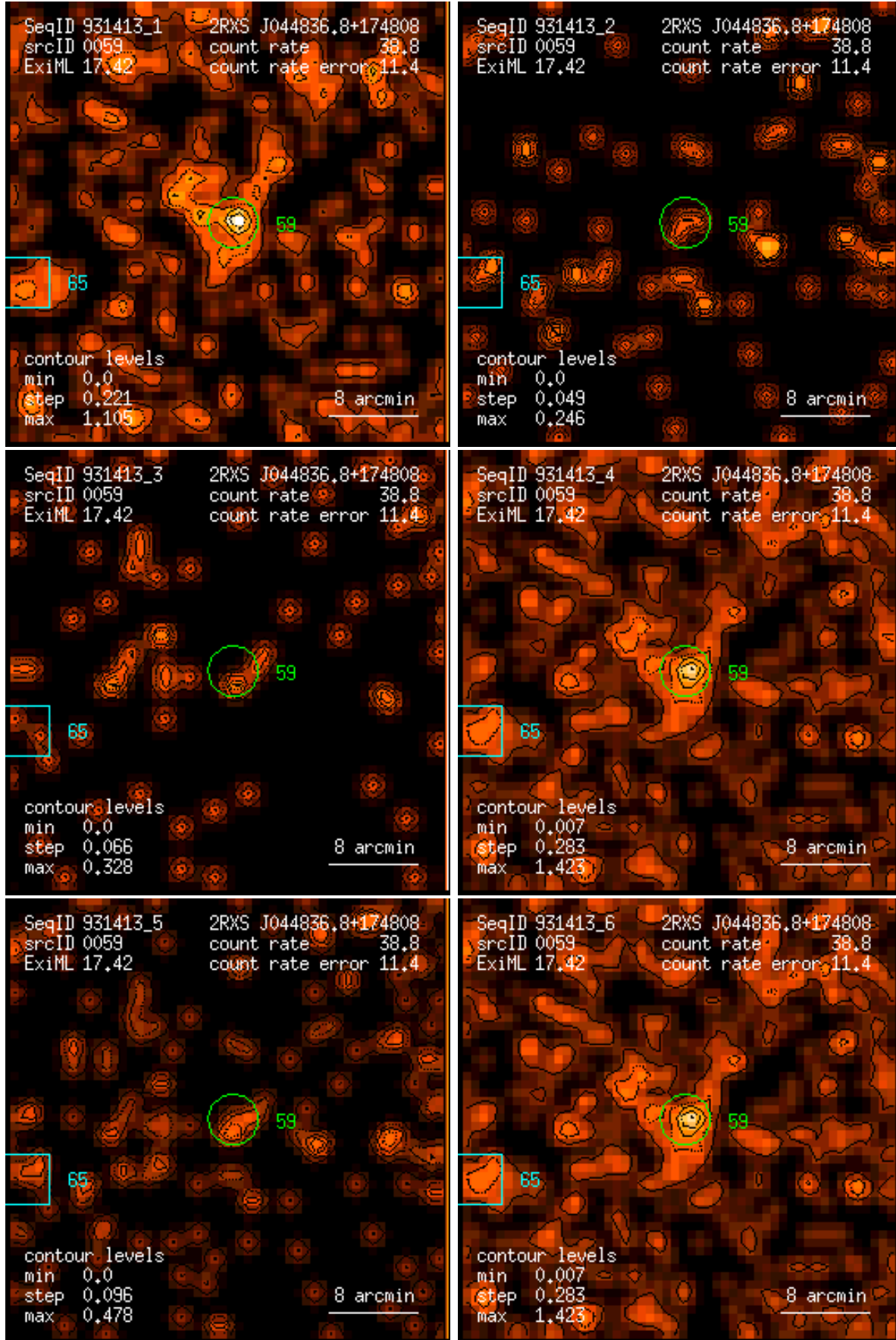
Figure 59: RASS 931413: detection 0059: band rate images, Gaussian filter: (1) PSPC channels 11 – 41, (2) 52 – 90, (3) 91 – 201, (4) 11 – 235, (5) 52 – 201, (6) 11 – 201. Broad band rates in counts/ks. Band rate contour levels in counts/ks/arcmin 2 .
