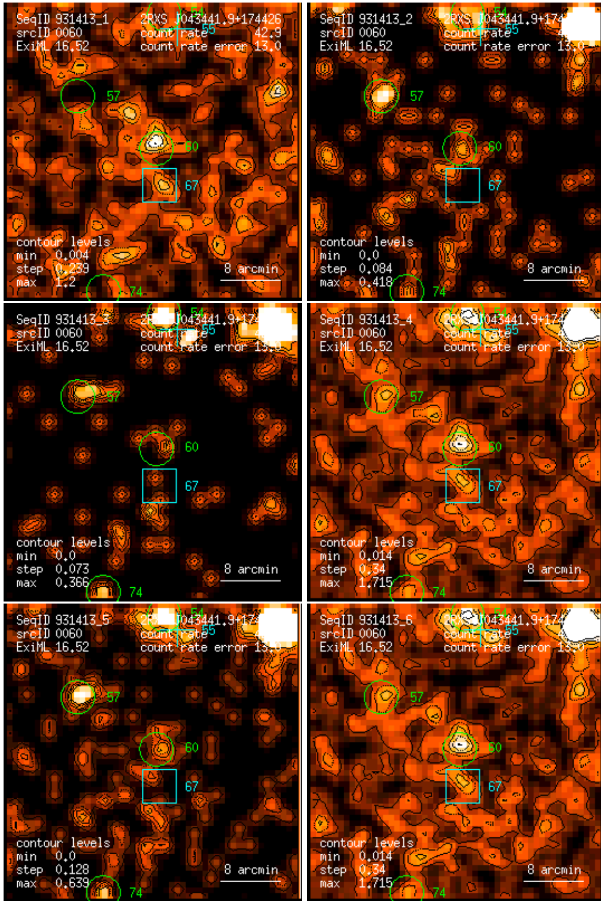
Figure 60: RASS 931413: detection 0060: band rate images, Gaussian filter: (1) PSPC channels 11 – 41, (2) 52 – 90, (3) 91 – 201, (4) 11 – 235, (5) 52 – 201, (6) 11 – 201. Broad band rates in counts/ks. Band rate contour levels in counts/ks/arcmin 2 .
