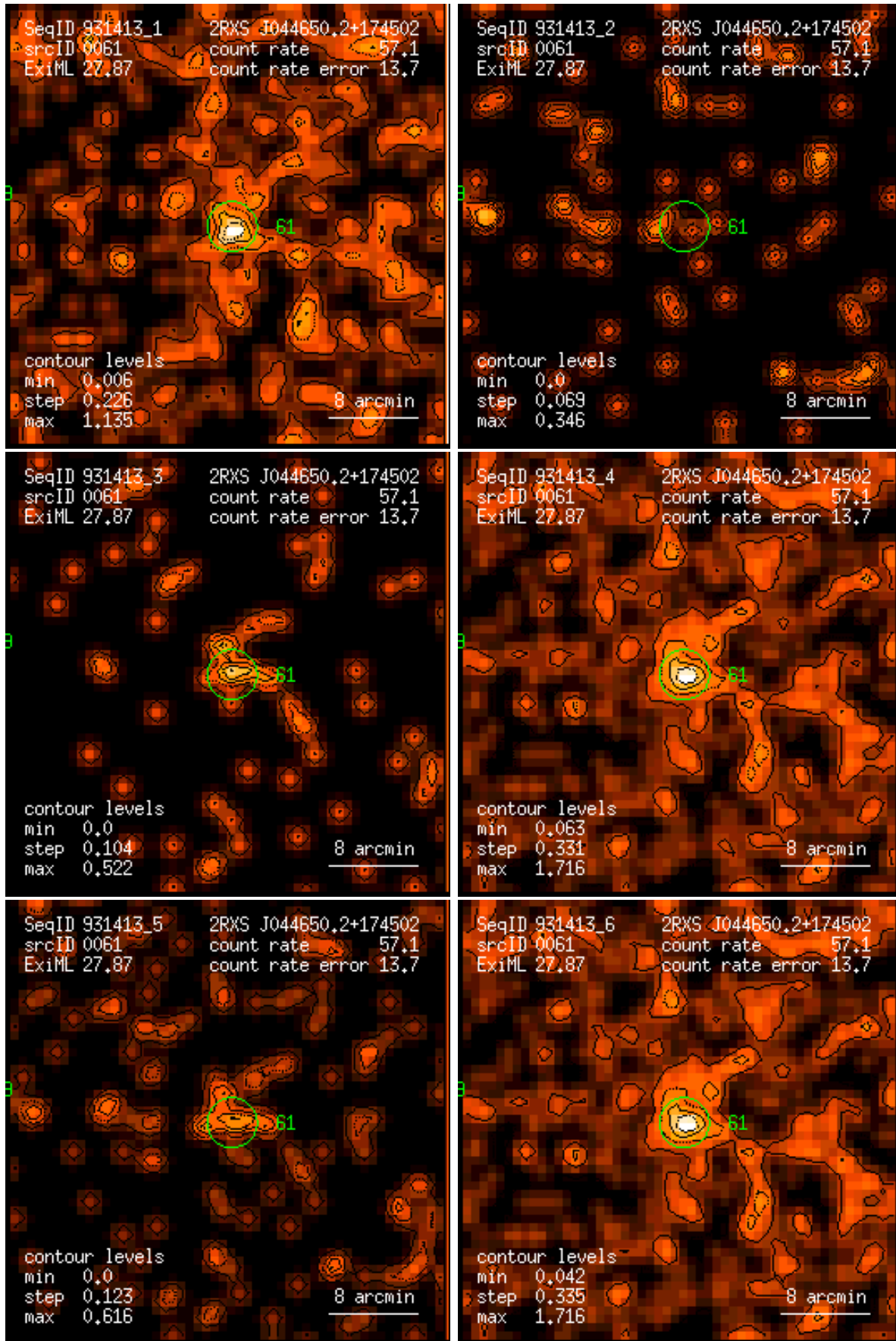
Figure 61: RASS 931413: detection 0061: band rate images, Gaussian filter: (1) PSPC channels 11 – 41, (2) 52 – 90, (3) 91 – 201, (4) 11 – 235, (5) 52 – 201, (6) 11 – 201. Broad band rates in counts/ks. Band rate contour levels in counts/ks/arcmin 2 .
