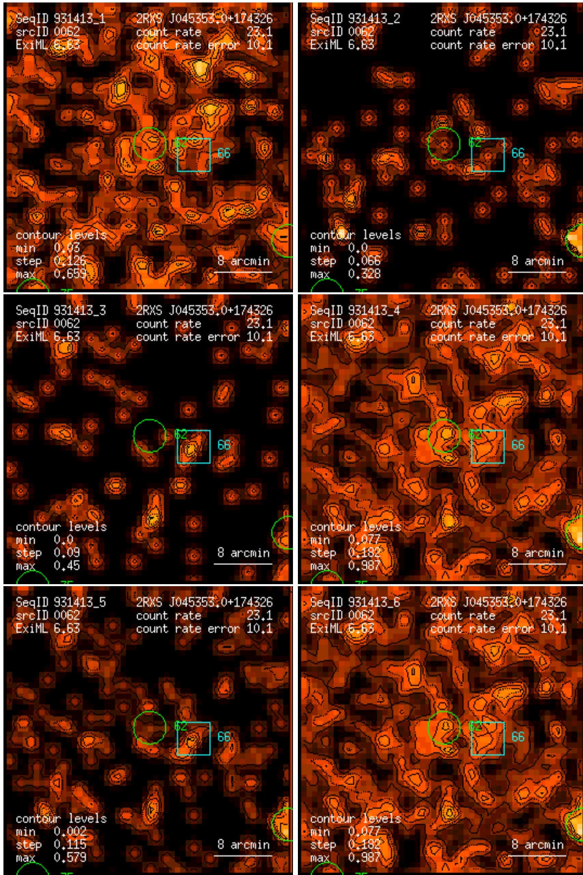
Figure 62: RASS 931413: detection 0062: band rate images, Gaussian filter: (1) PSPC channels 11 – 41, (2) 52 – 90, (3) 91 – 201, (4) 11 – 235, (5) 52 – 201, (6) 11 – 201. Broad band rates in counts/ks. Band rate contour levels in counts/ks/arcmin 2 .
