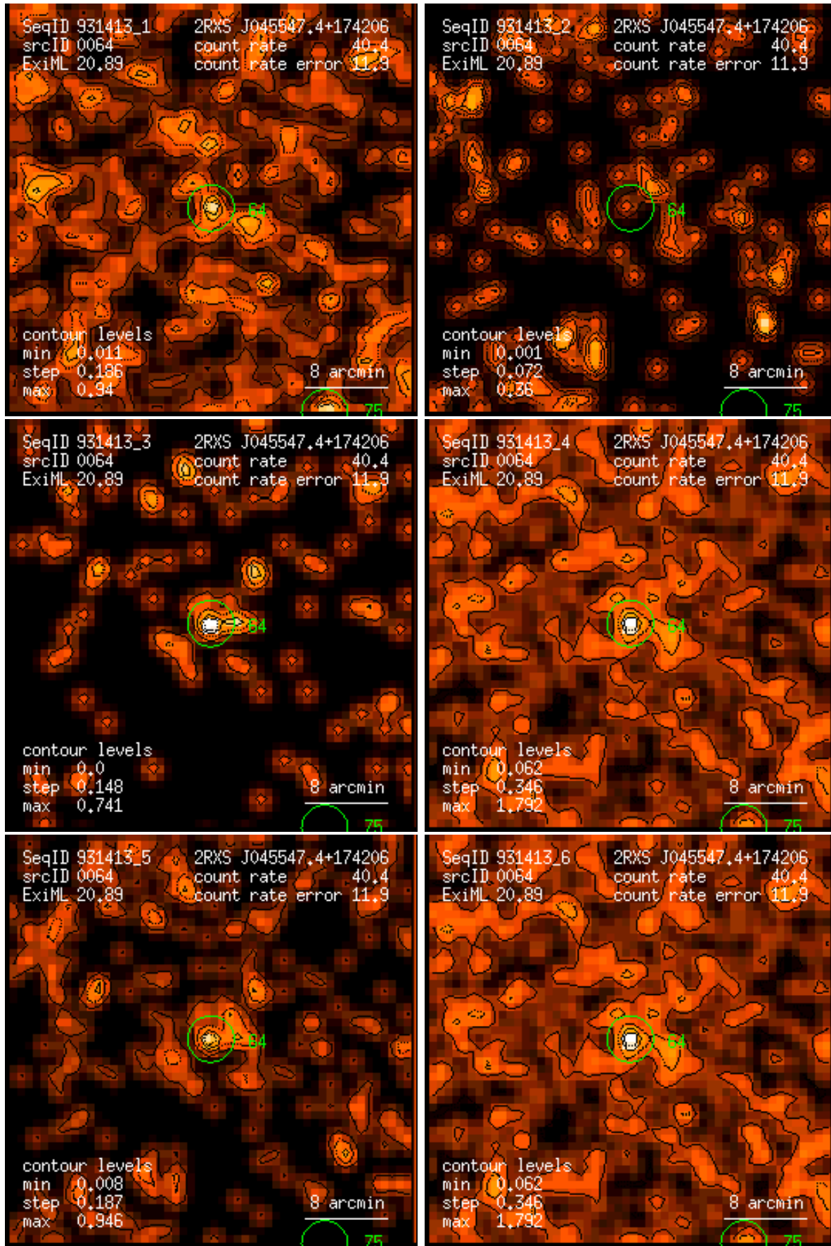
Figure 64: RASS 931413: detection 0064: band rate images, Gaussian filter: (1) PSPC channels 11 – 41, (2) 52 – 90, (3) 91 – 201, (4) 11 – 235, (5) 52 – 201, (6) 11 – 201. Broad band rates in counts/ks. Band rate contour levels in counts/ks/arcmin 2 .
