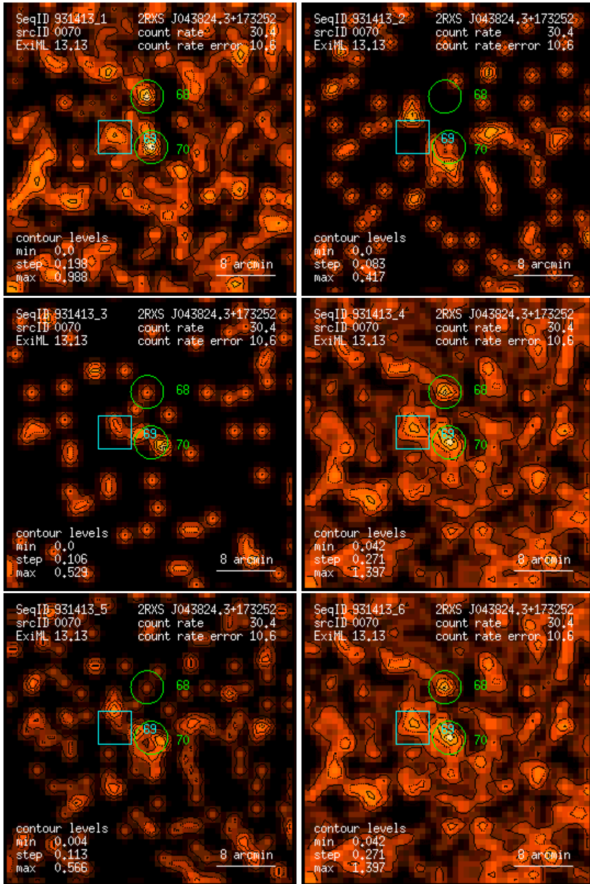
Figure 70: RASS 931413: detection 0070: band rate images, Gaussian filter: (1) PSPC channels 11 – 41, (2) 52 – 90, (3) 91 – 201, (4) 11 – 235, (5) 52 – 201, (6) 11 – 201. Broad band rates in counts/ks. Band rate contour levels in counts/ks/arcmin 2 .
