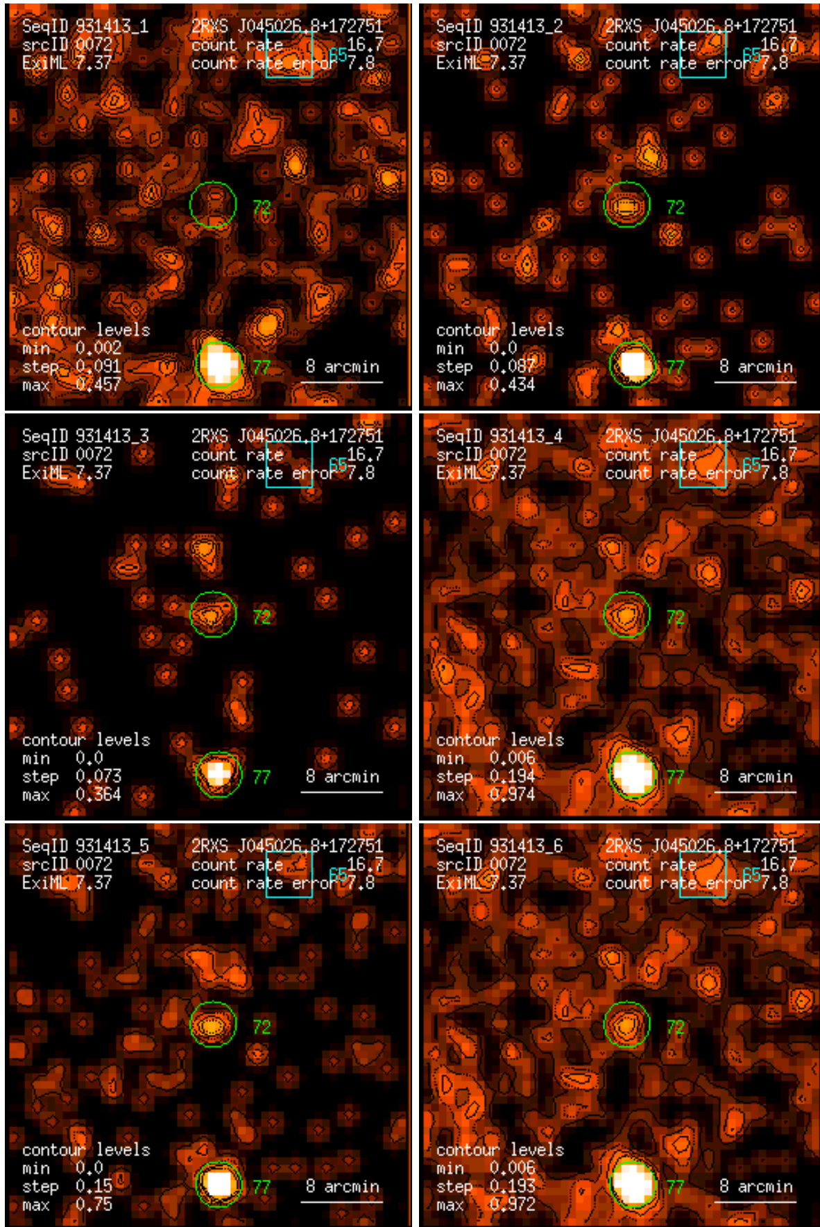
Figure 72: RASS 931413: detection 0072: band rate images, Gaussian filter: (1) PSPC channels 11 – 41, (2) 52 – 90, (3) 91 – 201, (4) 11 – 235, (5) 52 – 201, (6) 11 – 201. Broad band rates in counts/ks. Band rate contour levels in counts/ks/arcmin 2 .
