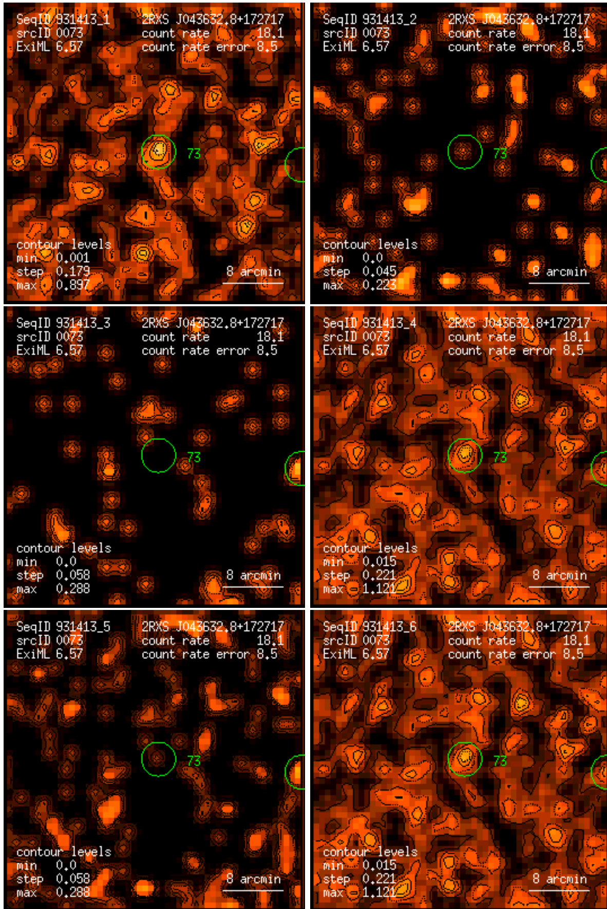
Figure 73: RASS 931413: detection 0073: band rate images, Gaussian filter: (1) PSPC channels 11 – 41, (2) 52 – 90, (3) 91 – 201, (4) 11 – 235, (5) 52 – 201, (6) 11 – 201. Broad band rates in counts/ks. Band rate contour levels in counts/ks/arcmin 2 .
