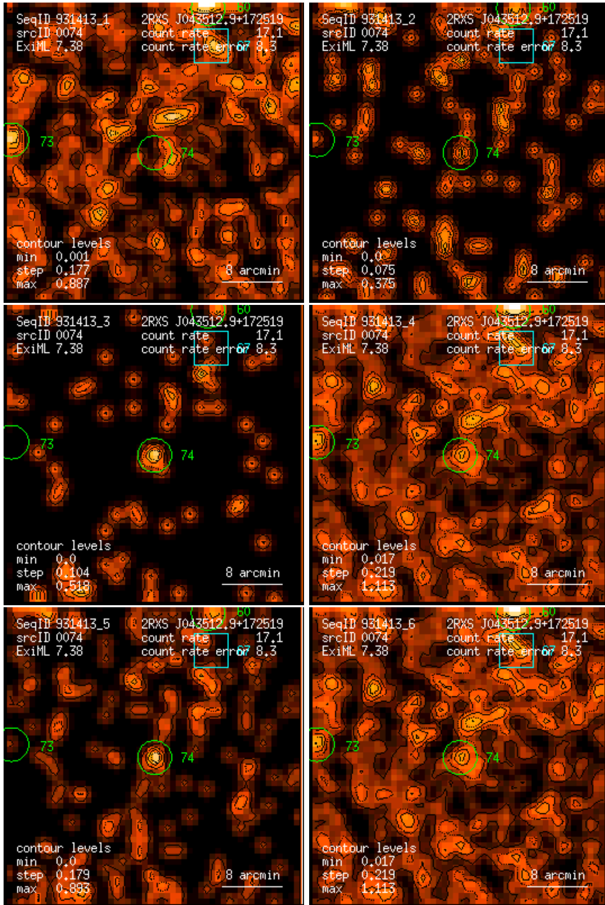
Figure 74: RASS 931413: detection 0074: band rate images, Gaussian filter: (1) PSPC channels 11 – 41, (2) 52 – 90, (3) 91 – 201, (4) 11 – 235, (5) 52 – 201, (6) 11 – 201. Broad band rates in counts/ks. Band rate contour levels in counts/ks/arcmin 2 .
