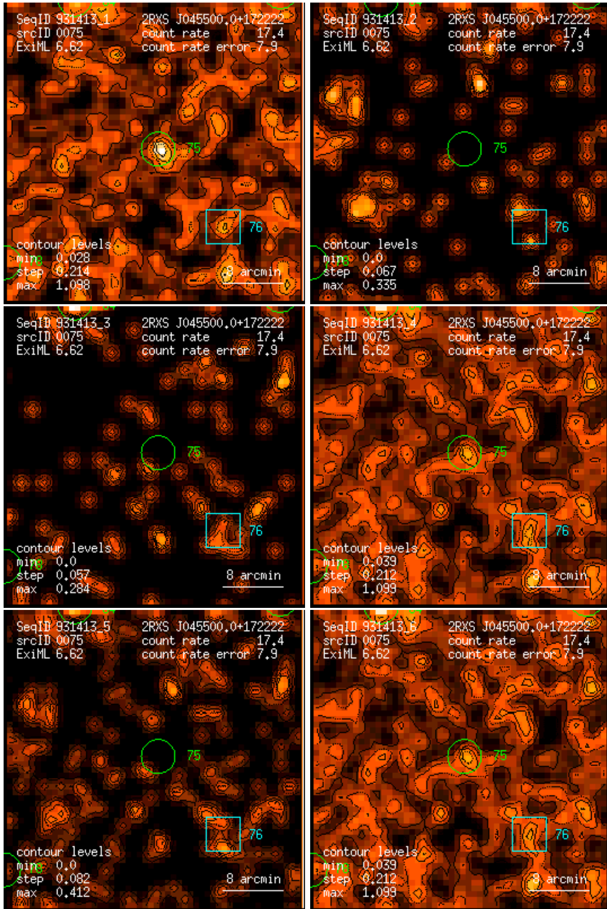
Figure 75: RASS 931413: detection 0075: band rate images, Gaussian filter: (1) PSPC channels 11 – 41, (2) 52 – 90, (3) 91 – 201, (4) 11 – 235, (5) 52 – 201, (6) 11 – 201. Broad band rates in counts/ks. Band rate contour levels in counts/ks/arcmin 2 .
