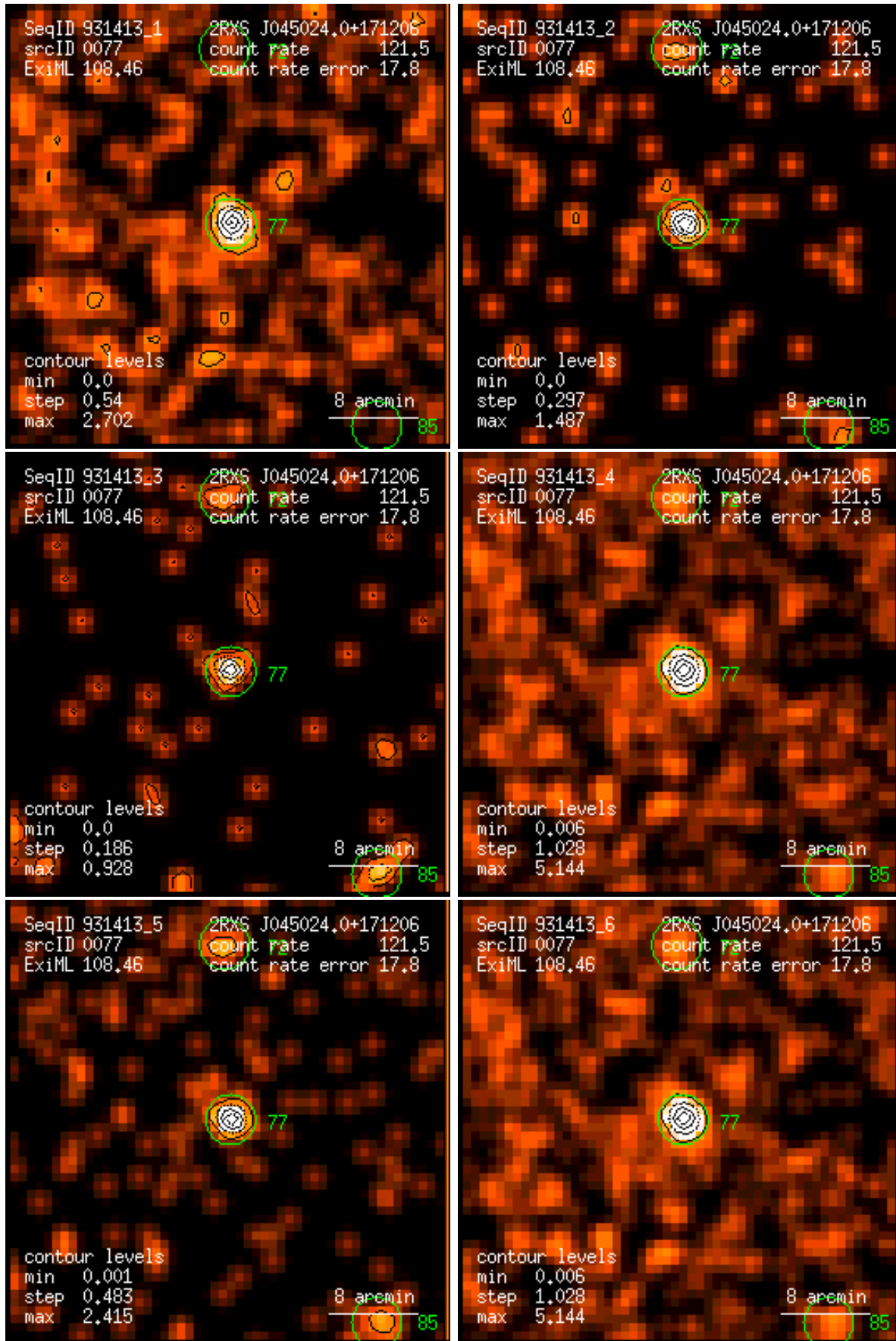
Figure 77: RASS 931413: detection 0077: band rate images, Gaussian filter: (1) PSPC channels 11 – 41, (2) 52 – 90, (3) 91 – 201, (4) 11 – 235, (5) 52 – 201, (6) 11 – 201. Broad band rates in counts/ks. Band rate contour levels in counts/ks/arcmin 2 .
