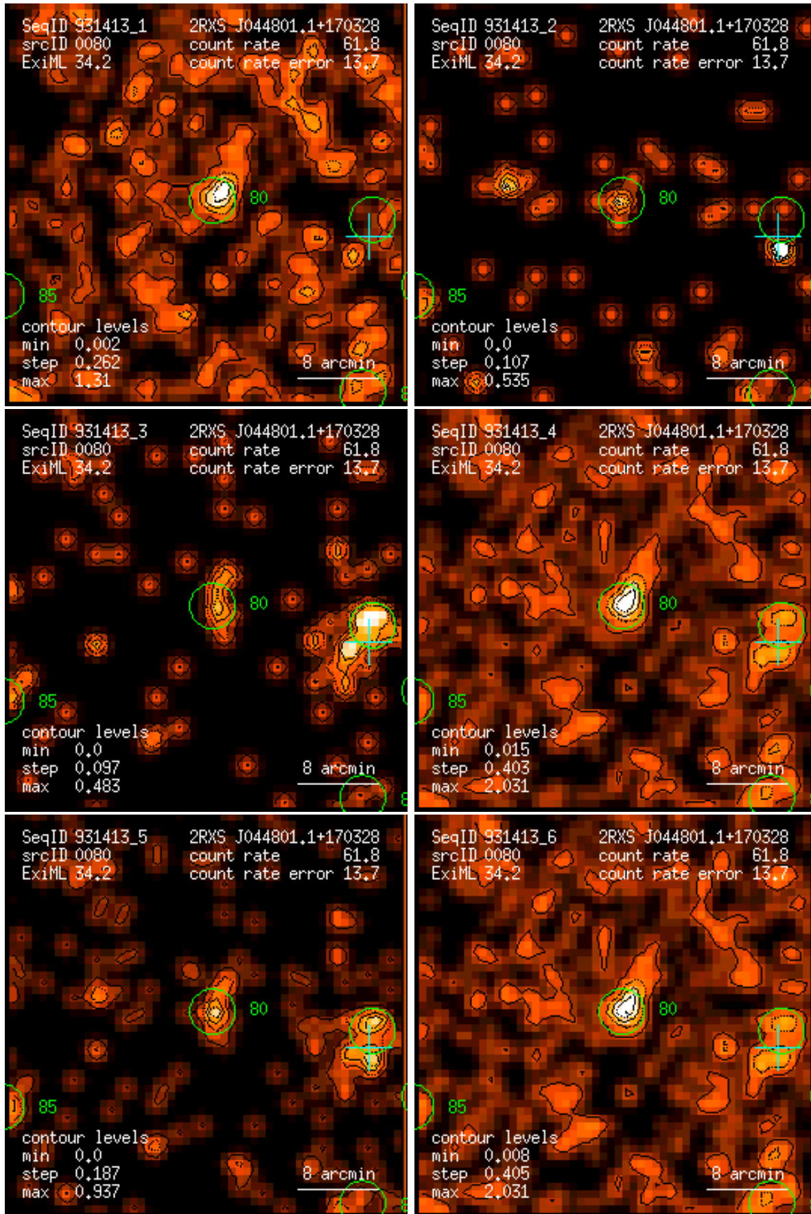
Figure 80: RASS 931413: detection 0080: band rate images, Gaussian filter: (1) PSPC channels 11 – 41, (2) 52 – 90, (3) 91 – 201, (4) 11 – 235, (5) 52 – 201, (6) 11 – 201. Broad band rates in counts/ks. Band rate contour levels in counts/ks/arcmin 2 .
