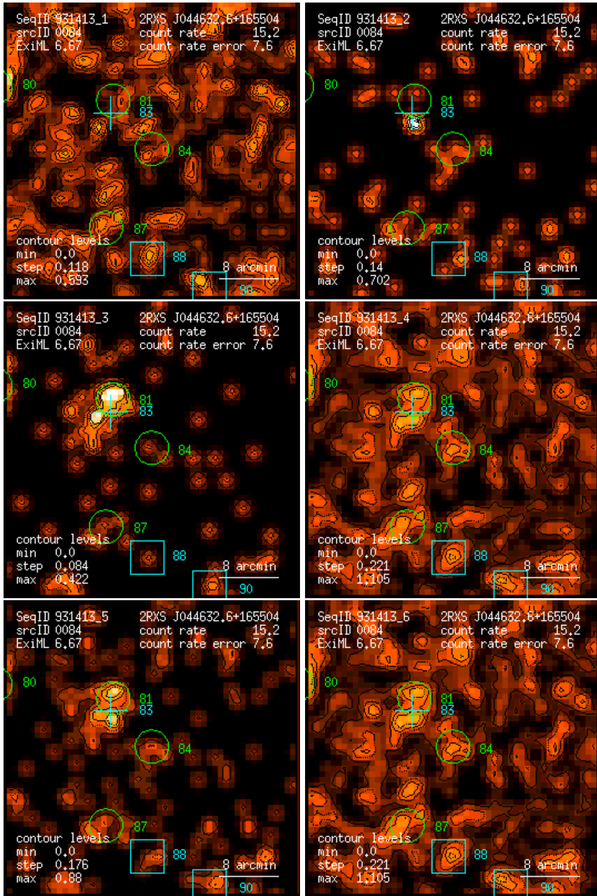
Figure 84: RASS 931413: detection 0084: band rate images, Gaussian filter: (1) PSPC channels 11 – 41, (2) 52 – 90, (3) 91 – 201, (4) 11 – 235, (5) 52 – 201, (6) 11 – 201. Broad band rates in counts/ks. Band rate contour levels in counts/ks/arcmin 2 .
