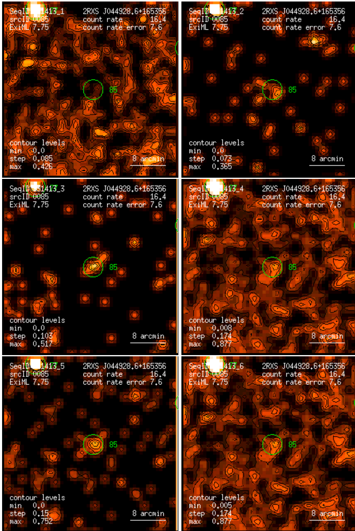
Figure 85: RASS 931413: detection 0085: band rate images, Gaussian filter: (1) PSPC channels 11 – 41, (2) 52 – 90, (3) 91 – 201, (4) 11 – 235, (5) 52 – 201, (6) 11 – 201. Broad band rates in counts/ks. Band rate contour levels in counts/ks/arcmin 2 .
