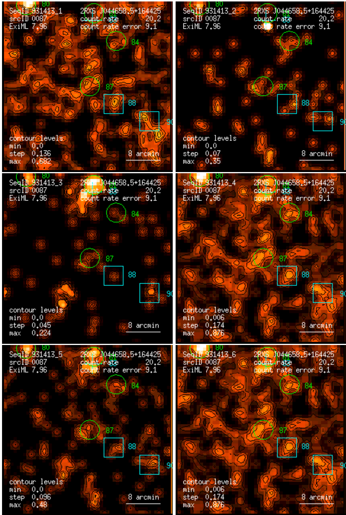
Figure 87: RASS 931413: detection 0087: band rate images, Gaussian filter: (1) PSPC channels 11 – 41, (2) 52 – 90, (3) 91 – 201, (4) 11 – 235, (5) 52 – 201, (6) 11 – 201. Broad band rates in counts/ks. Band rate contour levels in counts/ks/arcmin 2 .
