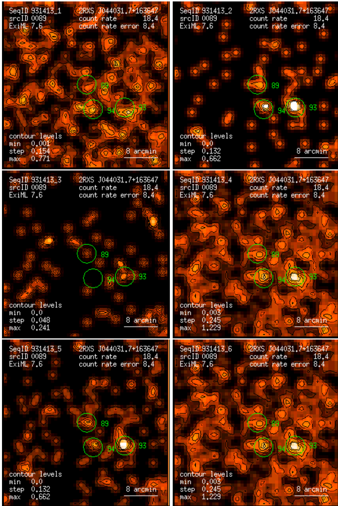
Figure 89: RASS 931413: detection 0089: band rate images, Gaussian filter: (1) PSPC channels 11 – 41, (2) 52 – 90, (3) 91 – 201, (4) 11 – 235, (5) 52 – 201, (6) 11 – 201. Broad band rates in counts/ks. Band rate contour levels in counts/ks/arcmin 2 .
