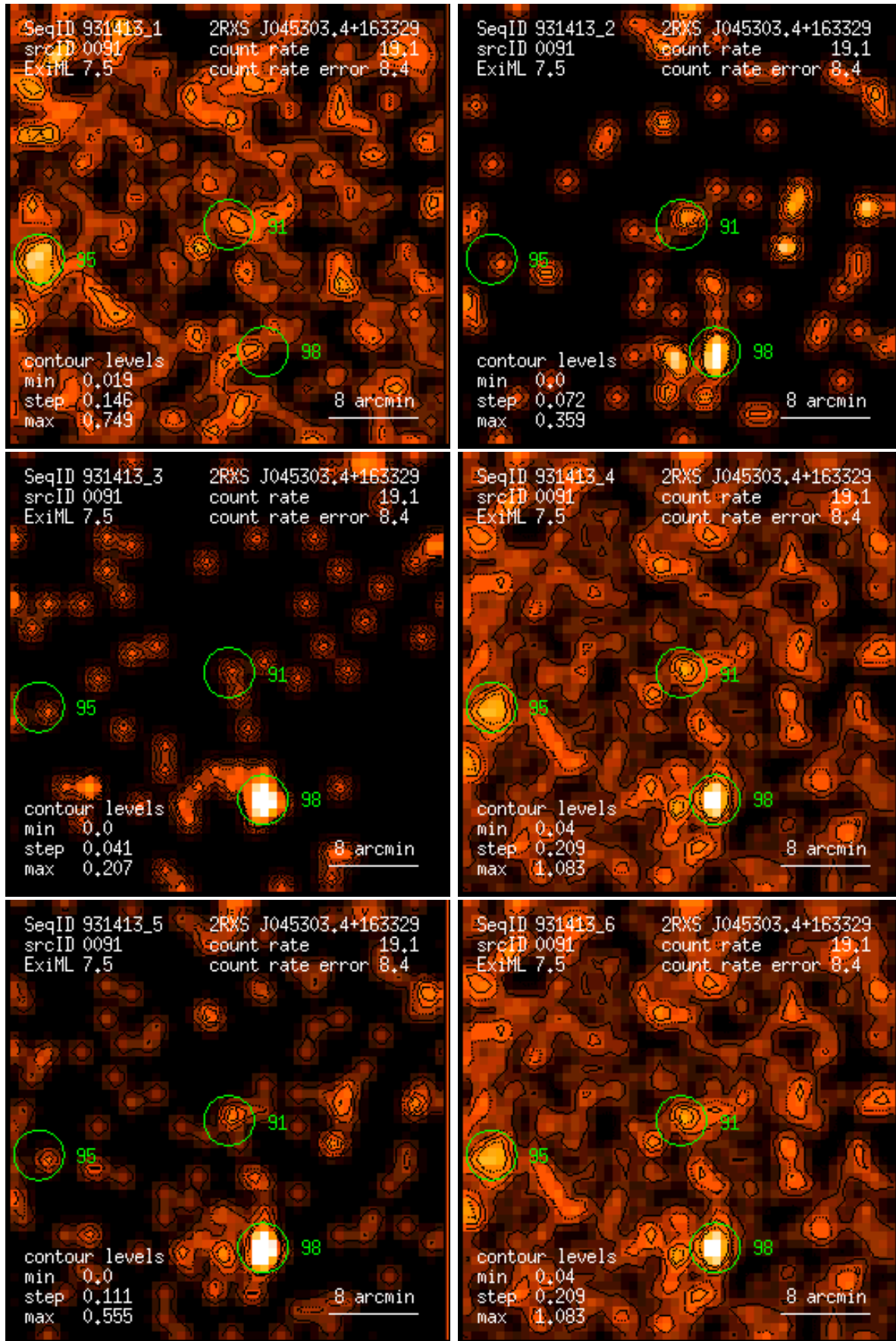
Figure 91: RASS 931413: detection 0091: band rate images, Gaussian filter: (1) PSPC channels 11 – 41, (2) 52 – 90, (3) 91 – 201, (4) 11 – 235, (5) 52 – 201, (6) 11 – 201. Broad band rates in counts/ks. Band rate contour levels in counts/ks/arcmin 2 .
