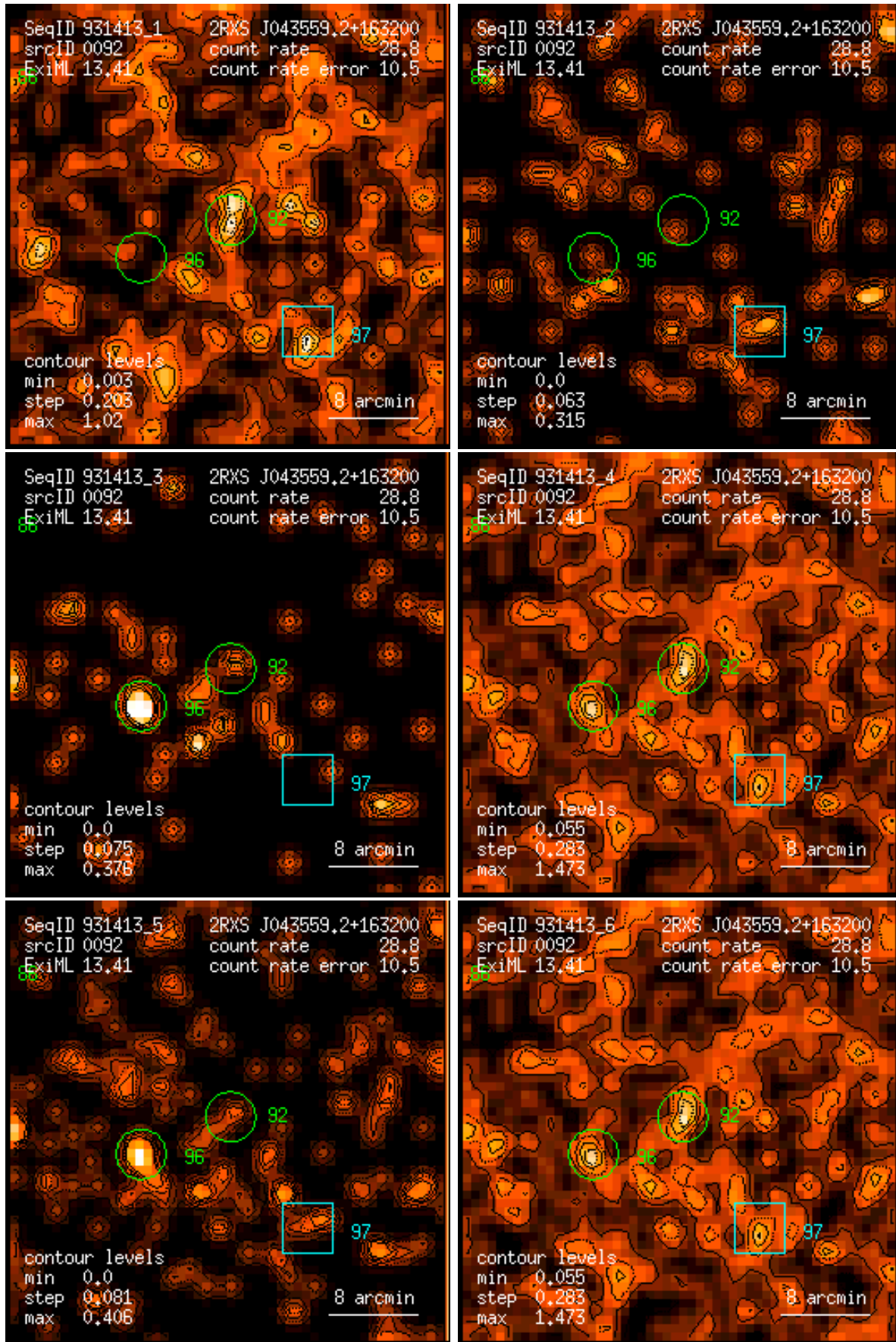
Figure 92: RASS 931413: detection 0092: band rate images, Gaussian filter: (1) PSPC channels 11 – 41, (2) 52 – 90, (3) 91 – 201, (4) 11 – 235, (5) 52 – 201, (6) 11 – 201. Broad band rates in counts/ks. Band rate contour levels in counts/ks/arcmin 2 .
