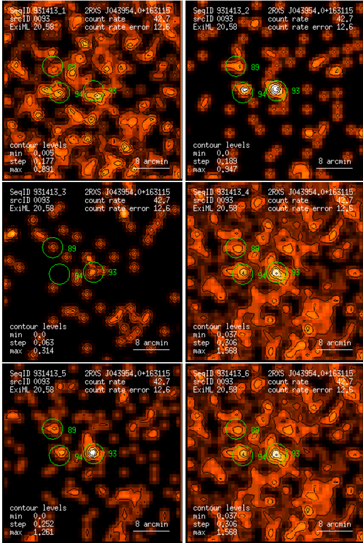
Figure 93: RASS 931413: detection 0093: band rate images, Gaussian filter: (1) PSPC channels 11 – 41, (2) 52 – 90, (3) 91 – 201, (4) 11 – 235, (5) 52 – 201, (6) 11 – 201. Broad band rates in counts/ks. Band rate contour levels in counts/ks/arcmin 2 .
