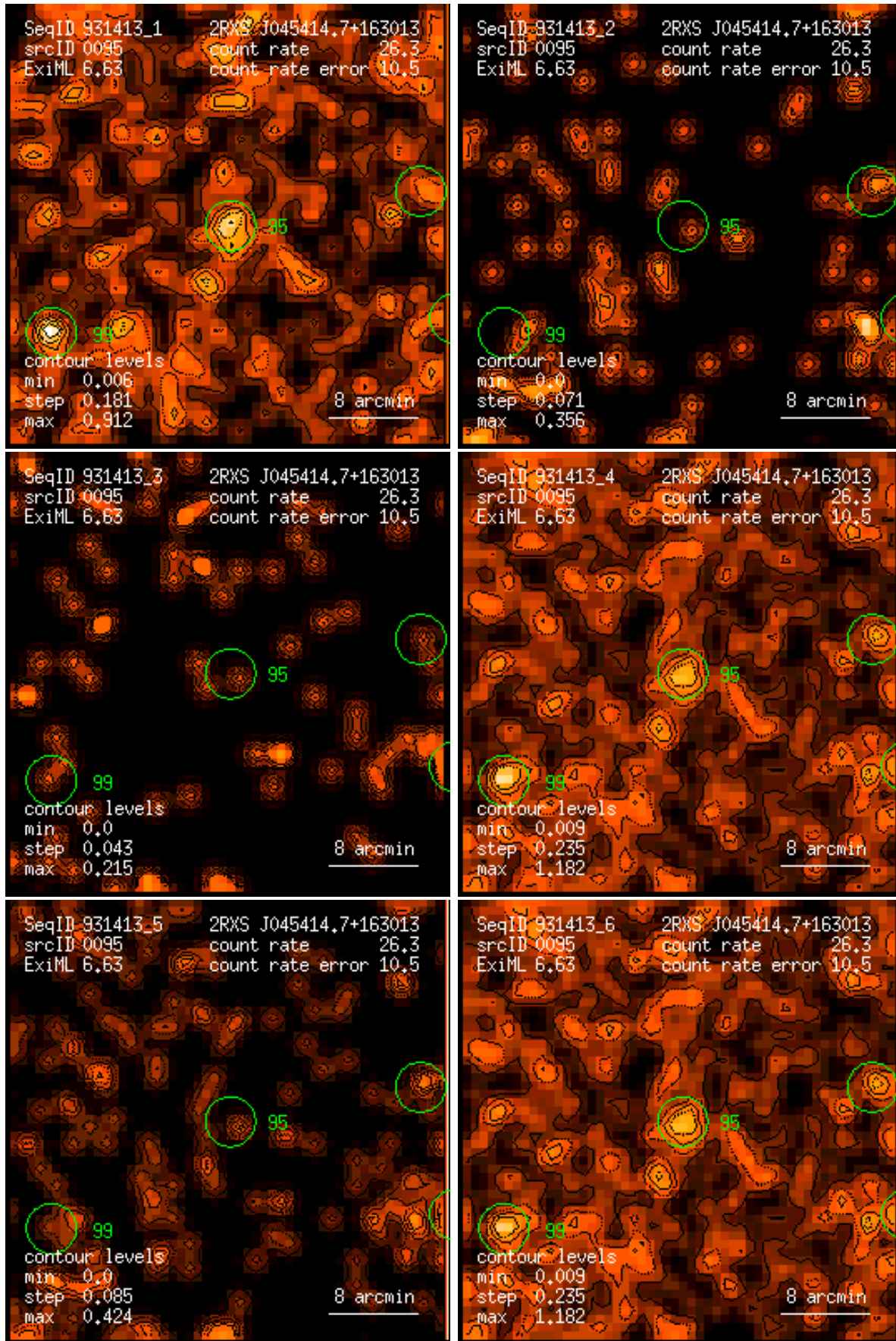
Figure 95: RASS 931413: detection 0095: band rate images, Gaussian filter: (1) PSPC channels 11 – 41, (2) 52 – 90, (3) 91 – 201, (4) 11 – 235, (5) 52 – 201, (6) 11 – 201. Broad band rates in counts/ks. Band rate contour levels in counts/ks/arcmin 2 .
