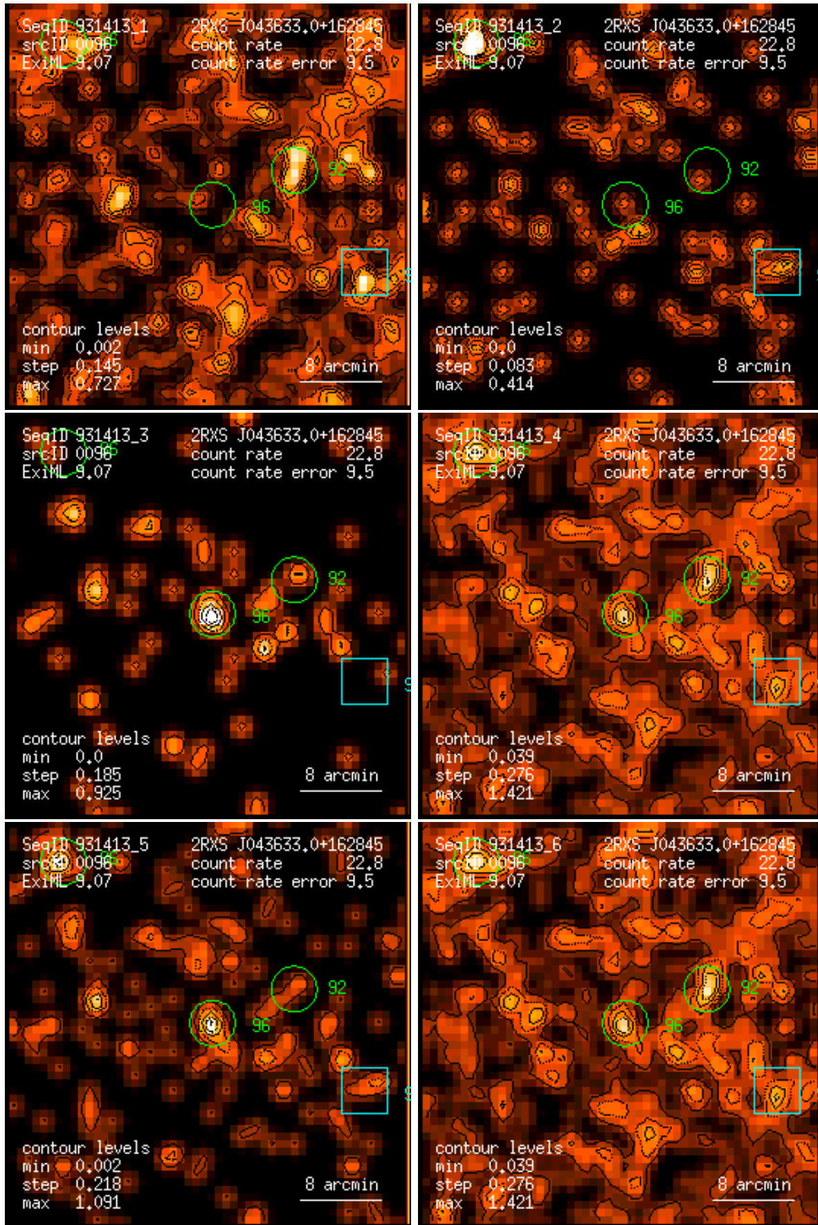
Figure 96: RASS 931413: detection 0096: band rate images, Gaussian filter: (1) PSPC channels 11 – 41, (2) 52 – 90, (3) 91 – 201, (4) 11 – 235, (5) 52 – 201, (6) 11 – 201. Broad band rates in counts/ks. Band rate contour levels in counts/ks/arcmin 2 .
