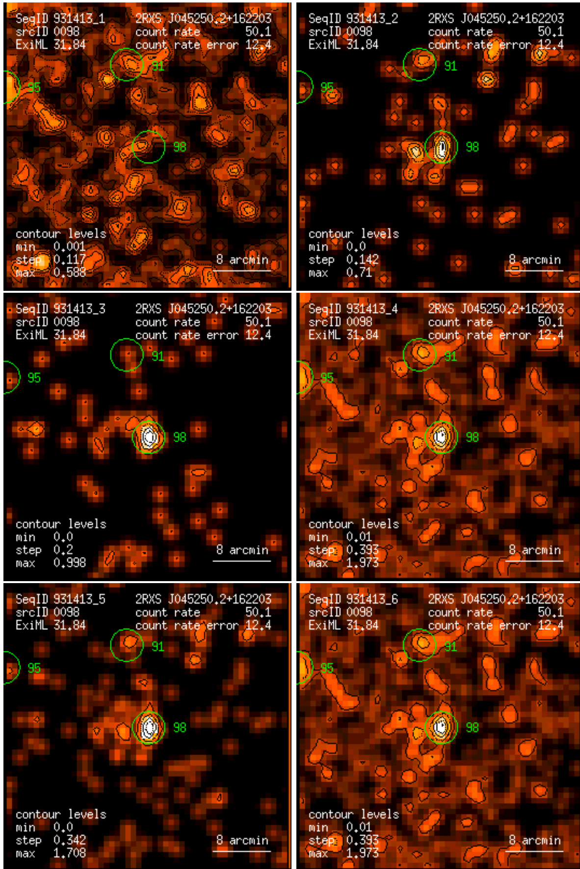
Figure 98: RASS 931413: detection 0098: band rate images, Gaussian filter: (1) PSPC channels 11 – 41, (2) 52 – 90, (3) 91 – 201, (4) 11 – 235, (5) 52 – 201, (6) 11 – 201. Broad band rates in counts/ks. Band rate contour levels in counts/ks/arcmin 2 .
