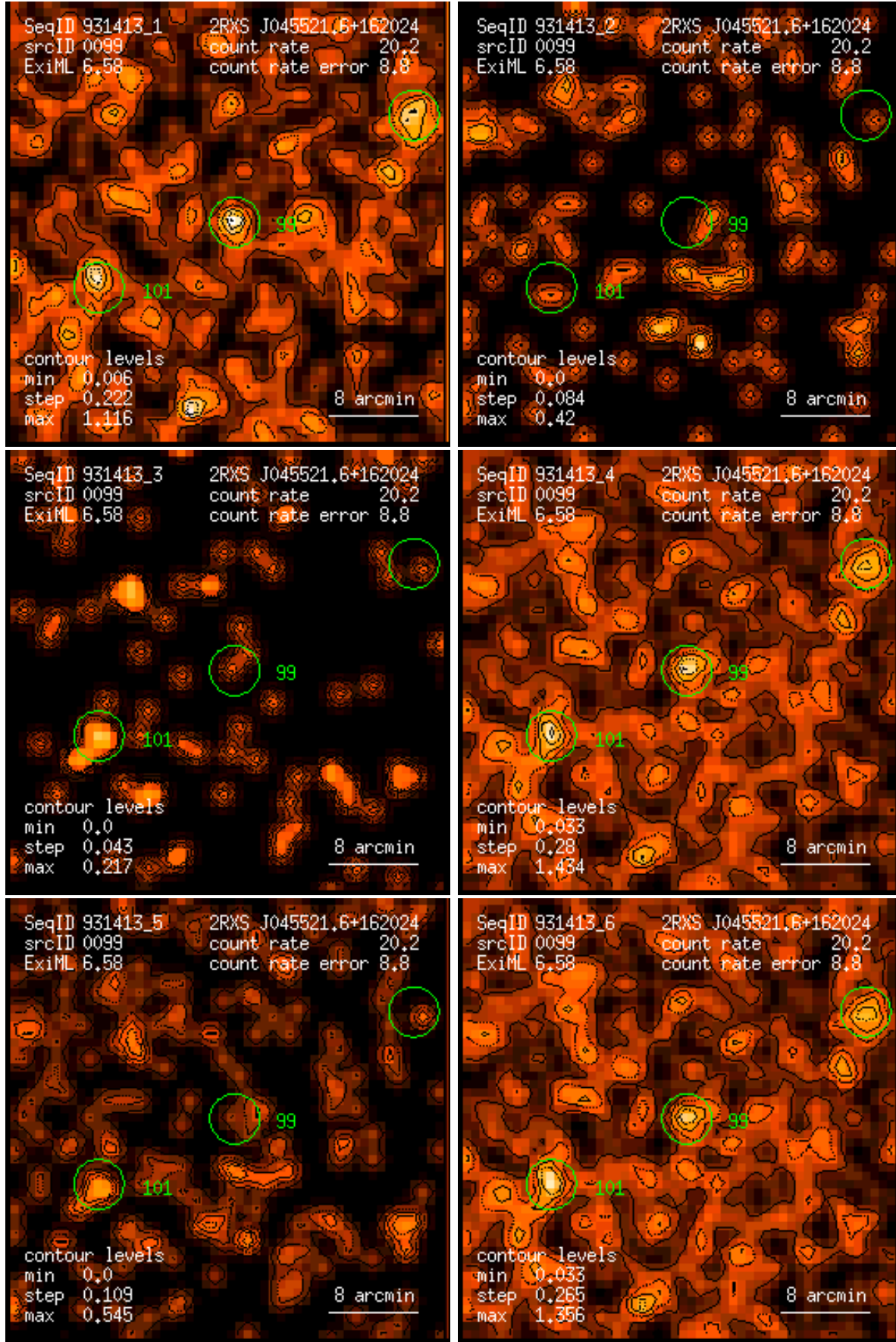
Figure 99: RASS 931413: detection 0099: band rate images, Gaussian filter: (1) PSPC channels 11 – 41, (2) 52 – 90, (3) 91 – 201, (4) 11 – 235, (5) 52 – 201, (6) 11 – 201. Broad band rates in counts/ks. Band rate contour levels in counts/ks/arcmin 2 .
