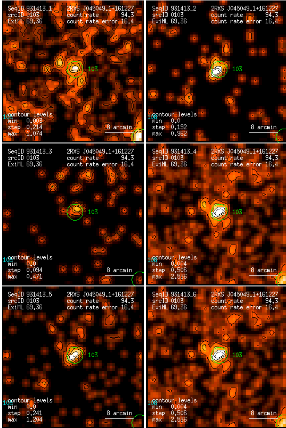
Figure 103: RASS 931413: detection 0103: band rate images, Gaussian filter: (1) PSPC channels 11 – 41, (2) 52 – 90, (3) 91 – 201, (4) 11 – 235, (5) 52 – 201, (6) 11 – 201. Broad band rates in counts/ks. Band rate contour levels in counts/ks/arcmin 2 .
